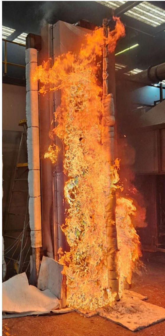
Figure 19 The specimen 6 minutes 22 seconds into the test (burner output at 200 kW)
