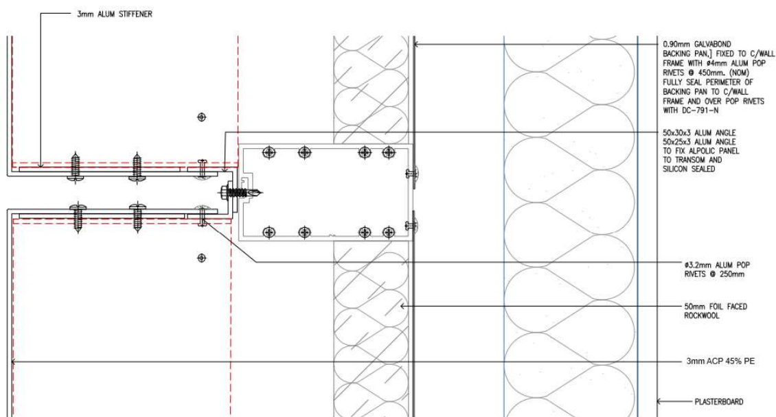
Figure 9 System assembly – middle join detail (D05)
