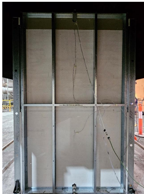
Figure 17 The specimen (unexposed side) before the reaction to fire test
