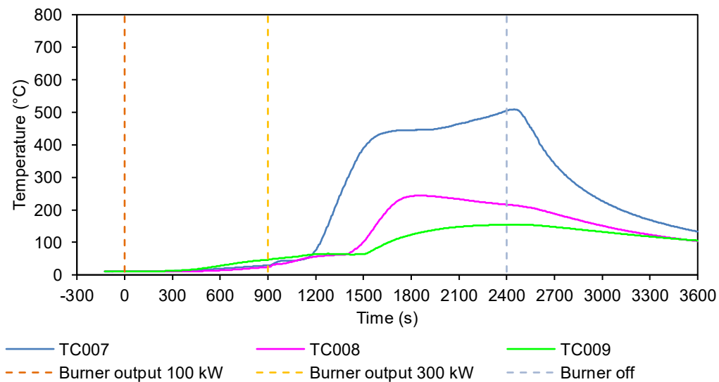
Figure 2 Cavity – Temperature vs time
