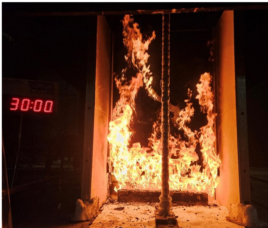
Figure 25 The specimen 30 minutes into the test (burner output at 300 kW)
