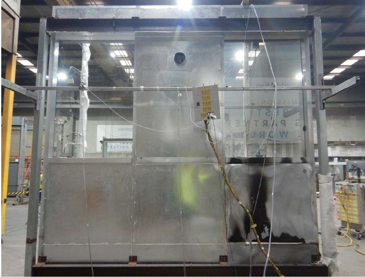
Figure 40 The specimen at end of test – unexposed side.
