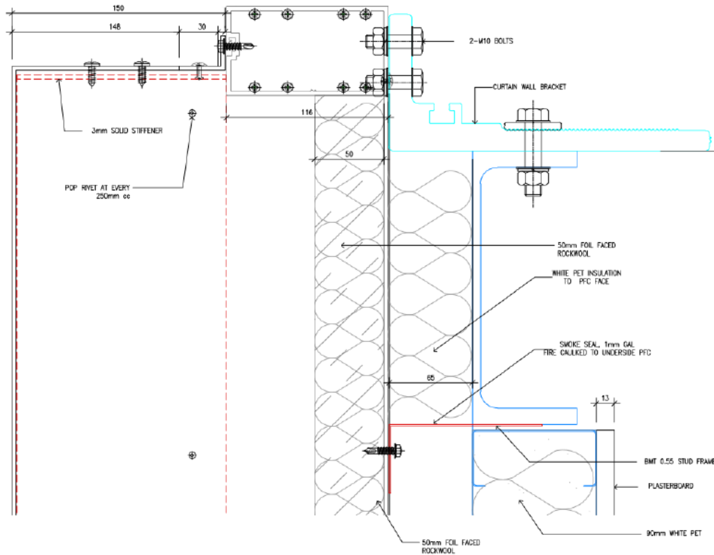
Figure 8 System assembly – top edge detail
