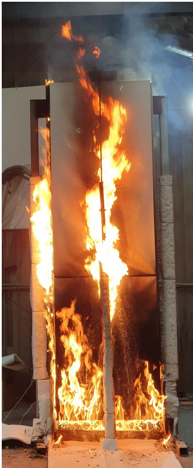
Figure 19 The specimen 19 minutes into the test (burner output at 200 kW)
