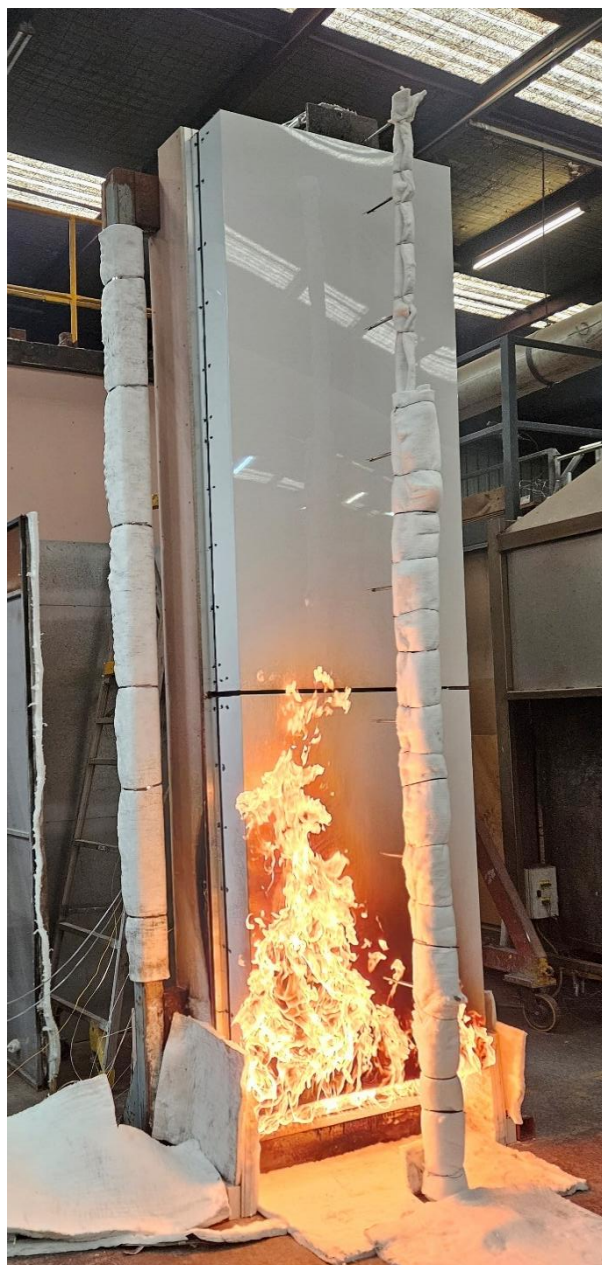
Figure 13 The specimen 2 minutes into the test (burner output at 200 kW)
