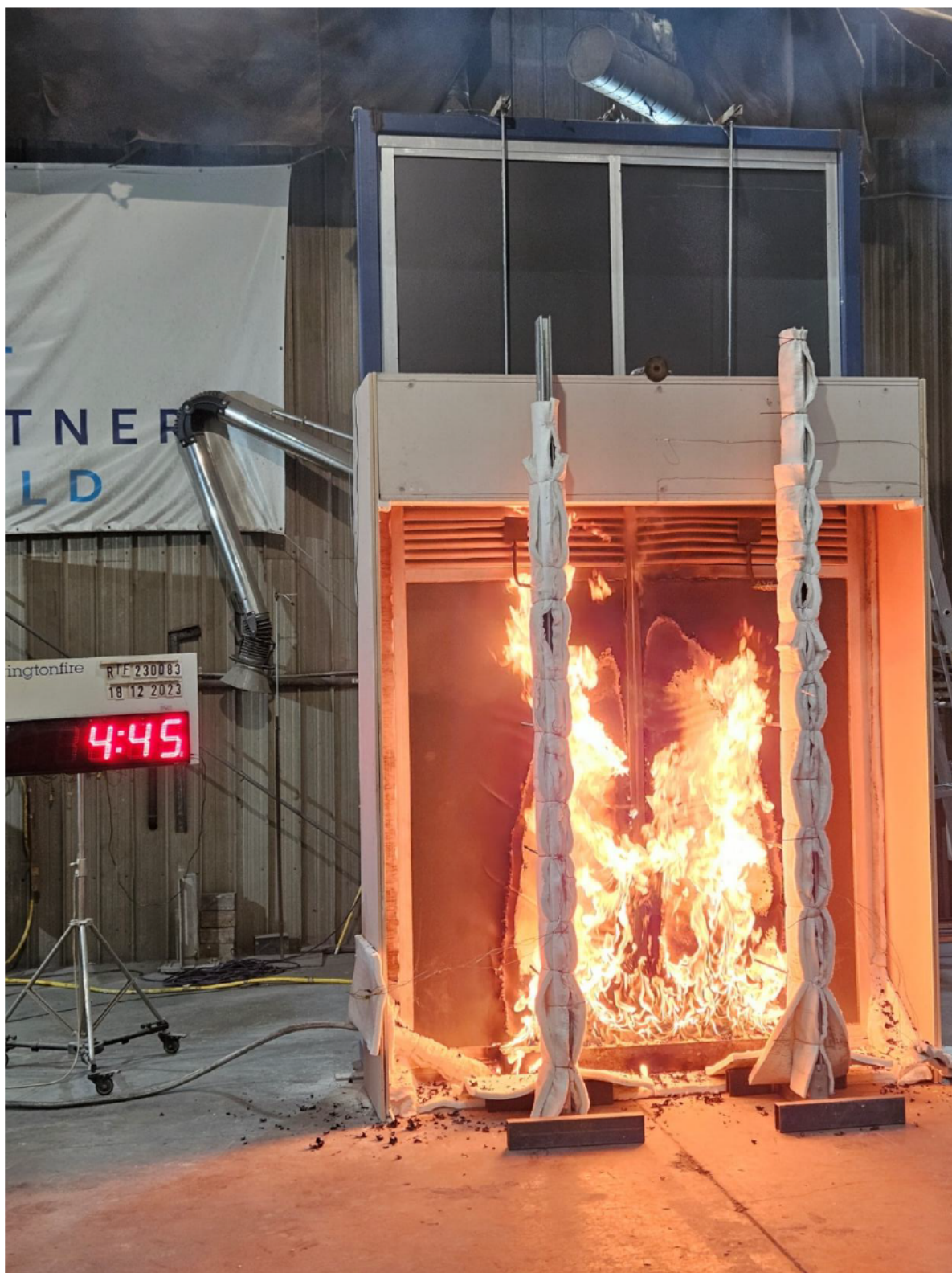
Figure 21 The specimen 4 minutes 45 seconds into the test
