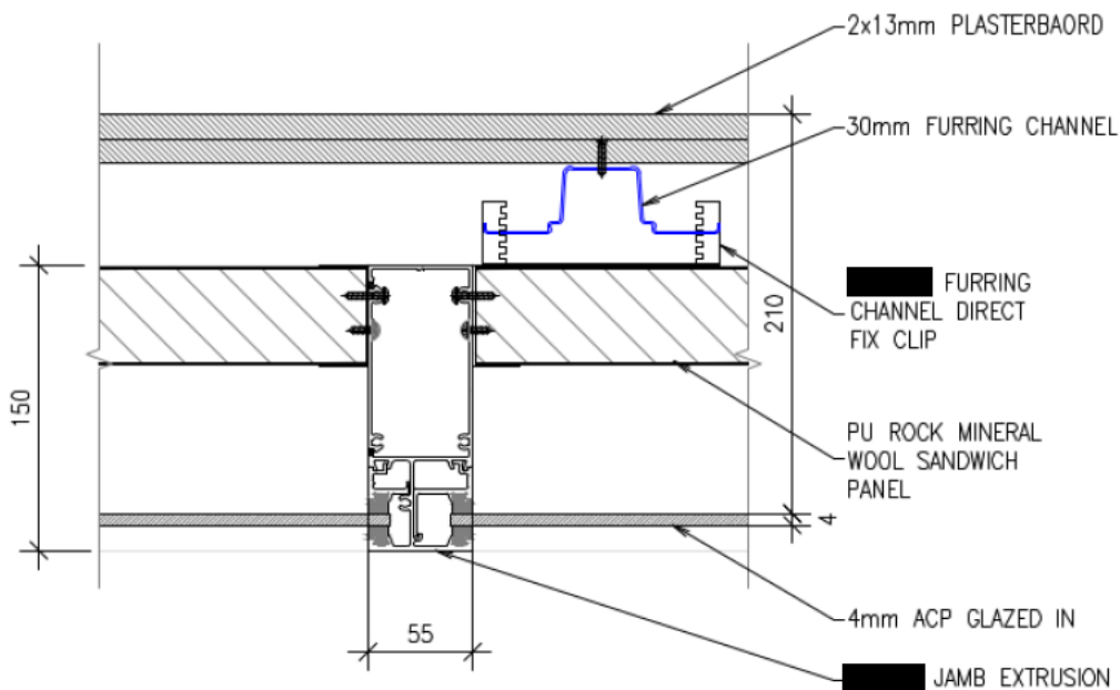
Figure 15 System detail – Detail D2
