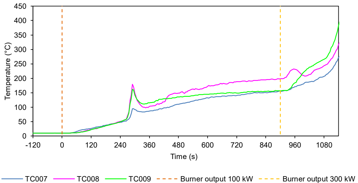
Figure 2 Cavity – Temperature vs time
