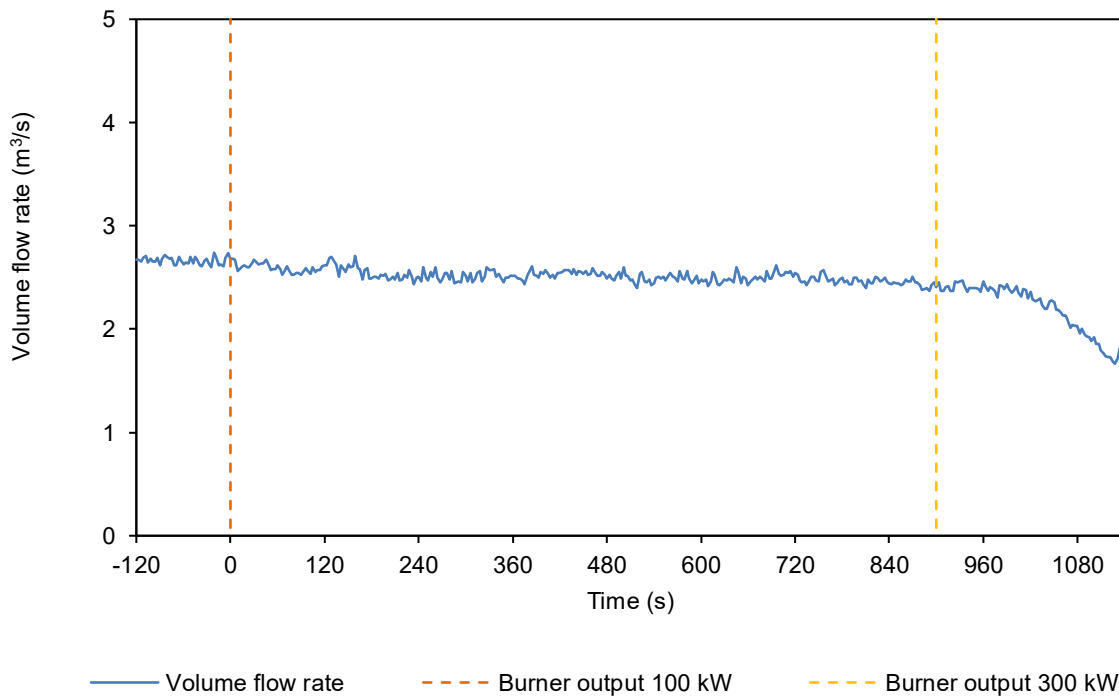
Figure 4 Volume flow rate in duct vs time
