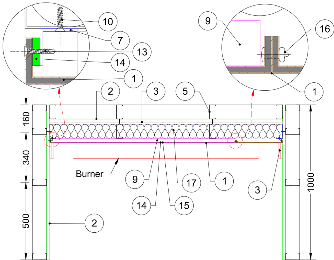
Figure 12 System assembly – Horizontal cross-section B-B
