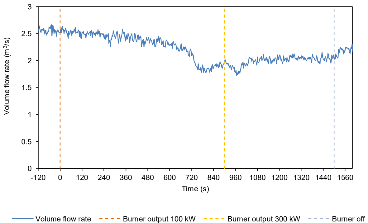
Figure 4 Volume flow rate in duct vs time
