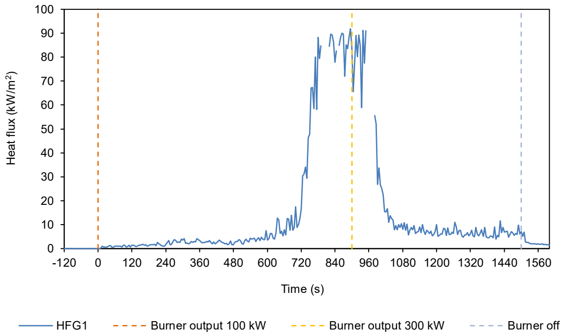
Figure 3 Heat flux vs time
