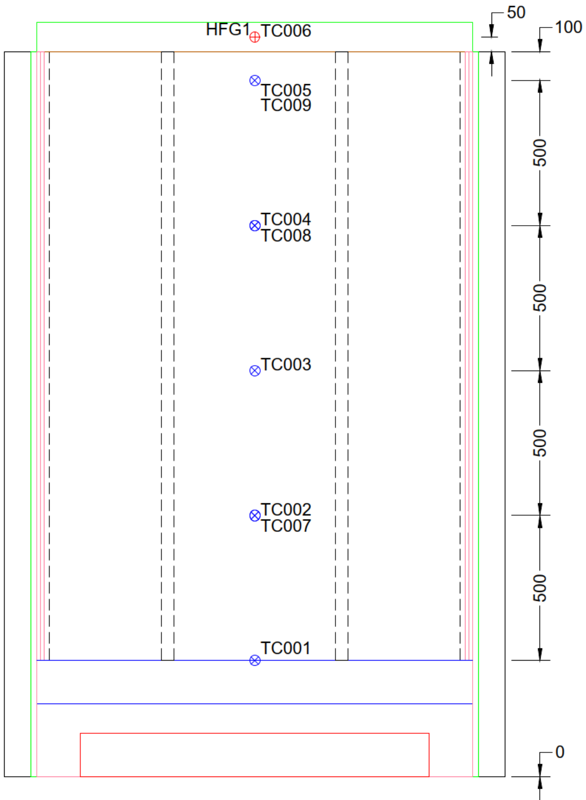
Figure 13 Instrumentation locations – Exposed side view
