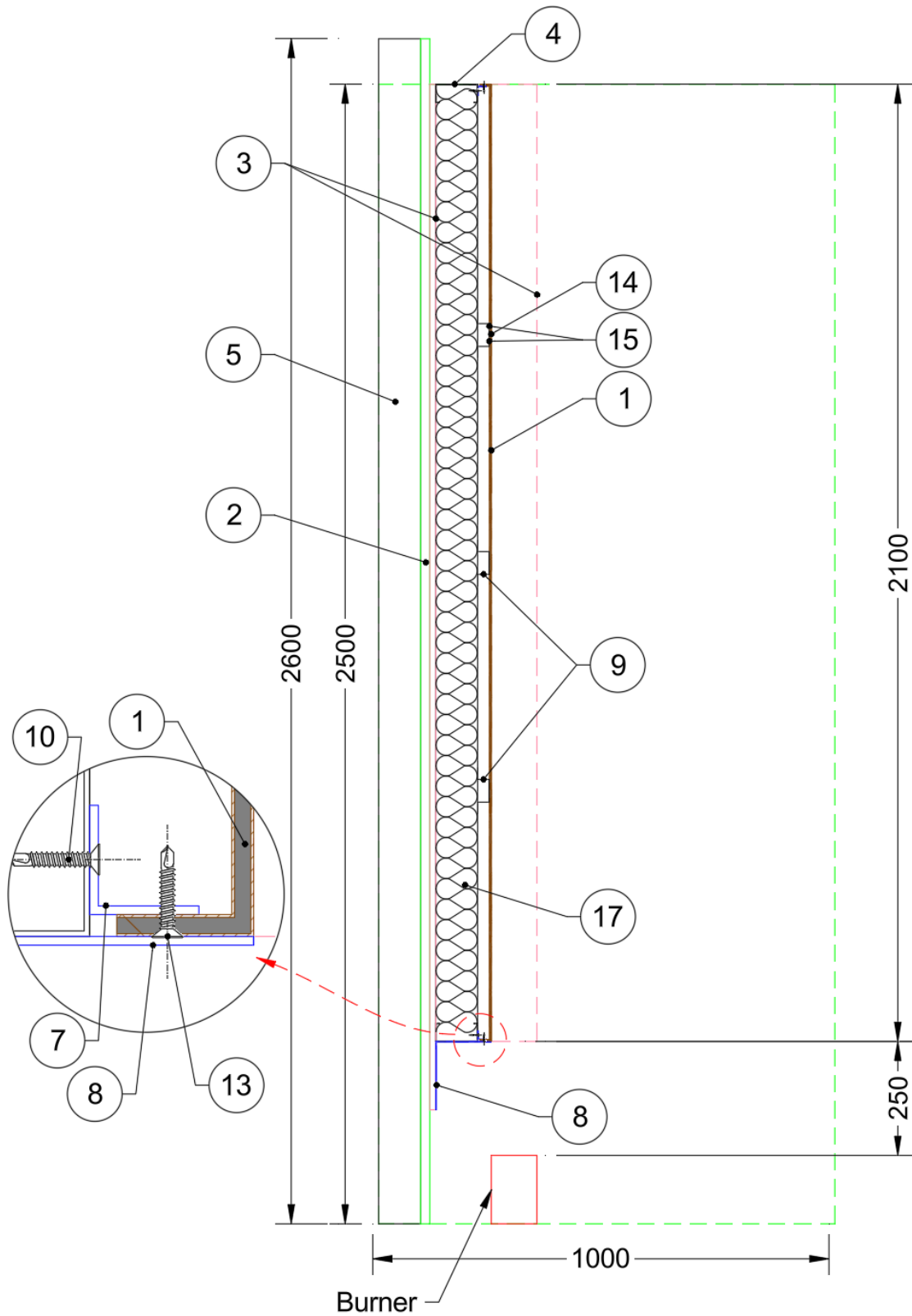
Figure 11 System assembly – Vertical cross-section A-A
