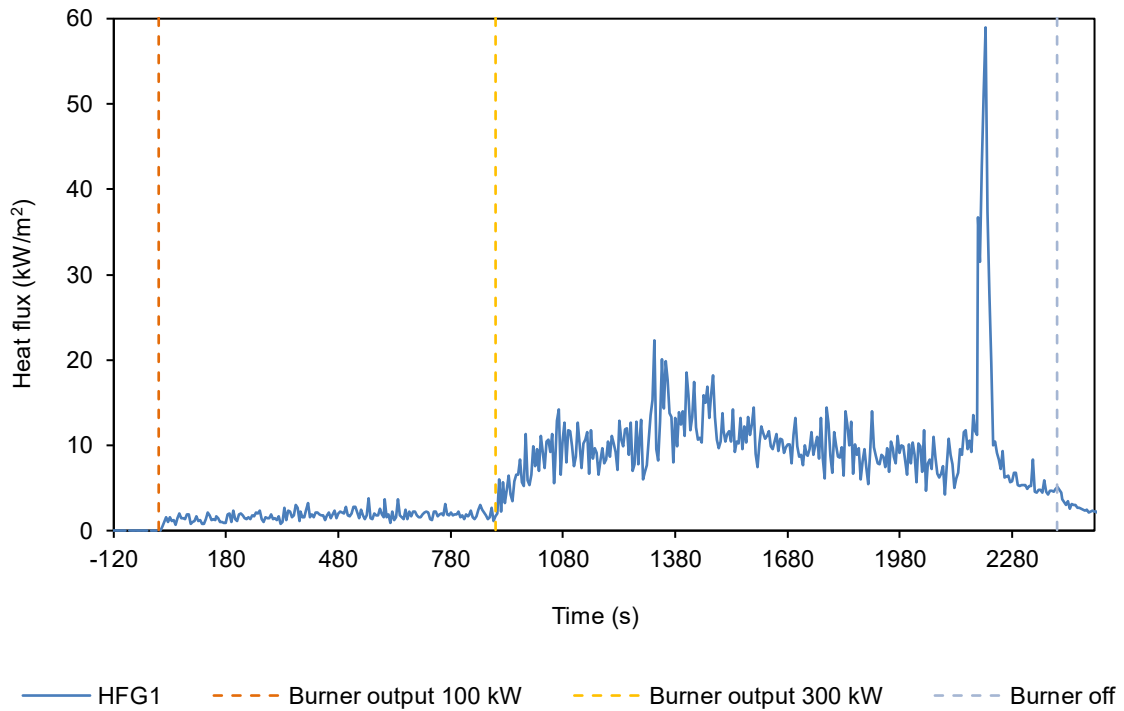
Figure 3 Heat flux vs time
