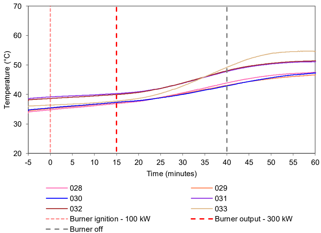
Figure 11 Internal temperatures of the back pan of module 4 (lower part) - Temperature vs. time.
