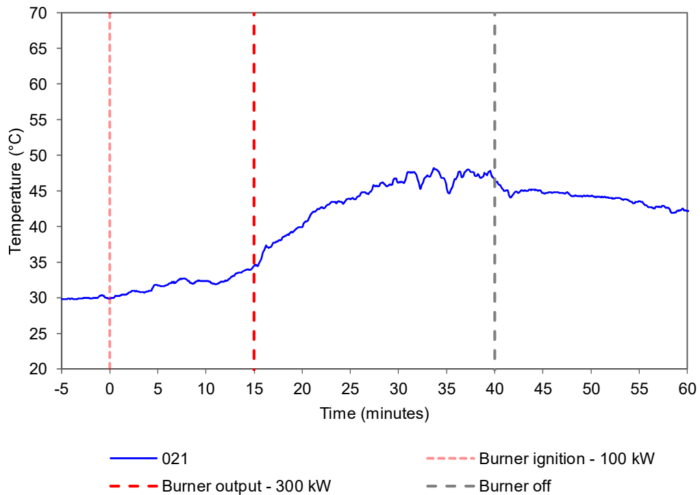
Figure 9 Internal temperature of the cavity of module 3 - Temperature vs. time.
