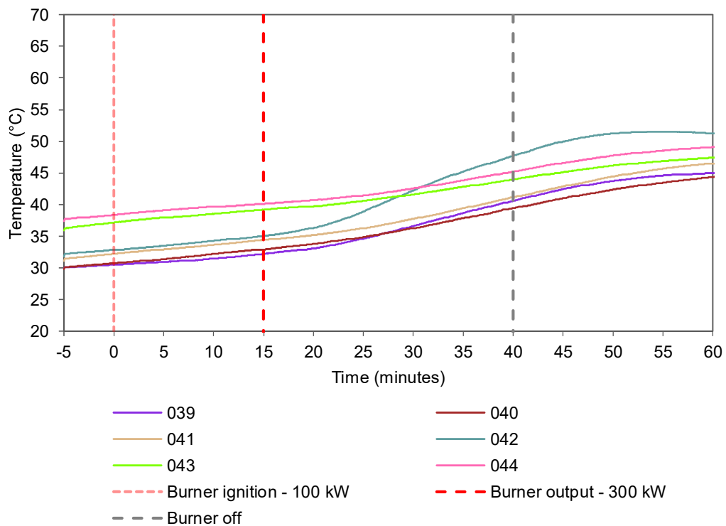
Figure 13 Internal temperatures of the back pan of module 5 (upper part) - Temperature vs. time.
