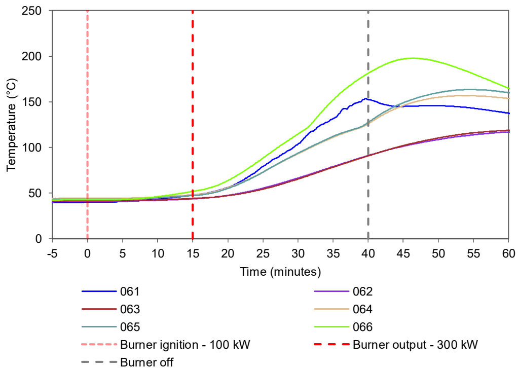
Figure 17 Internal temperatures of the back pan of module 6 - Temperature vs. time.
