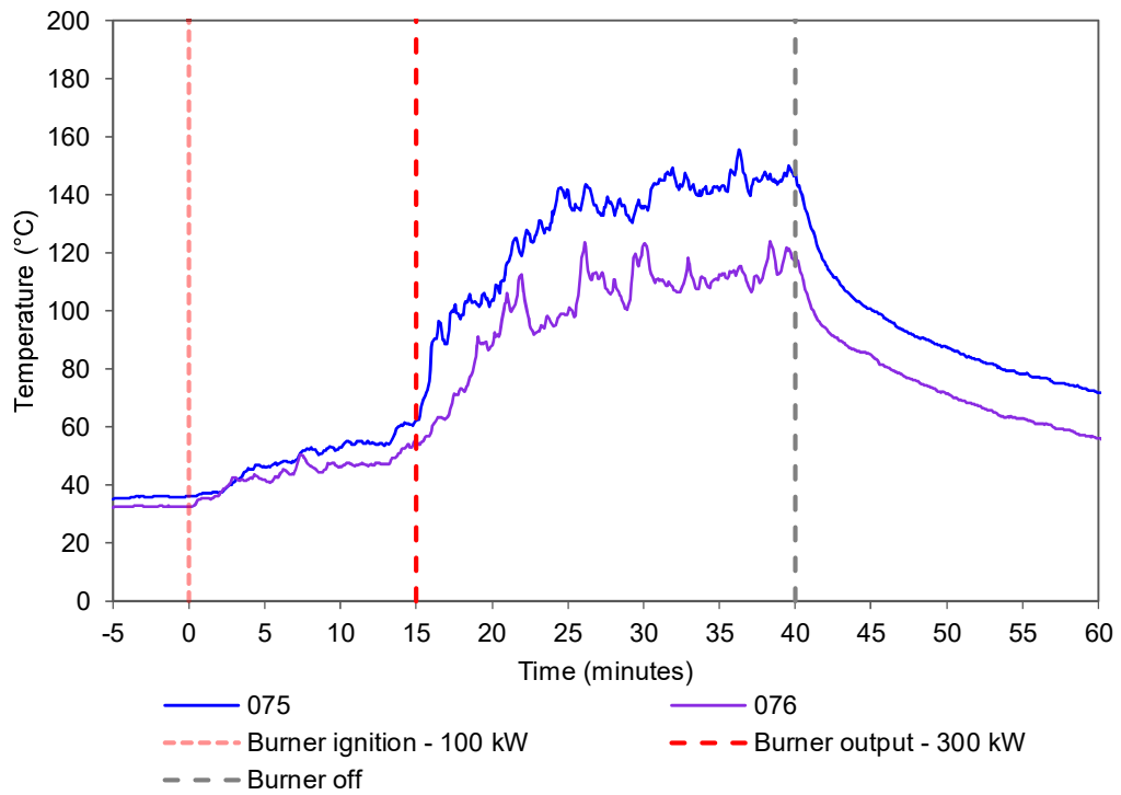
Figure 20 Internal temperatures of the cavity of module 7 - Temperature vs. time.
