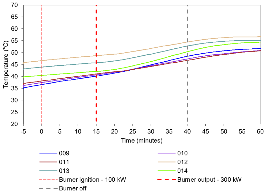
Figure 6 Internal temperatures of the back pan of module 2 - Temperature vs. time.
