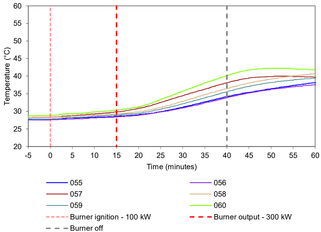
Figure 16 Internal temperatures of the back pan of module 8 - Temperature vs. time.
