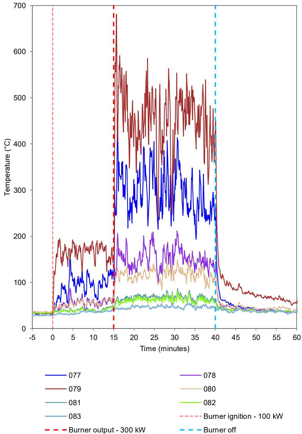
Figure 3 External temperatures - Temperature vs. time.
