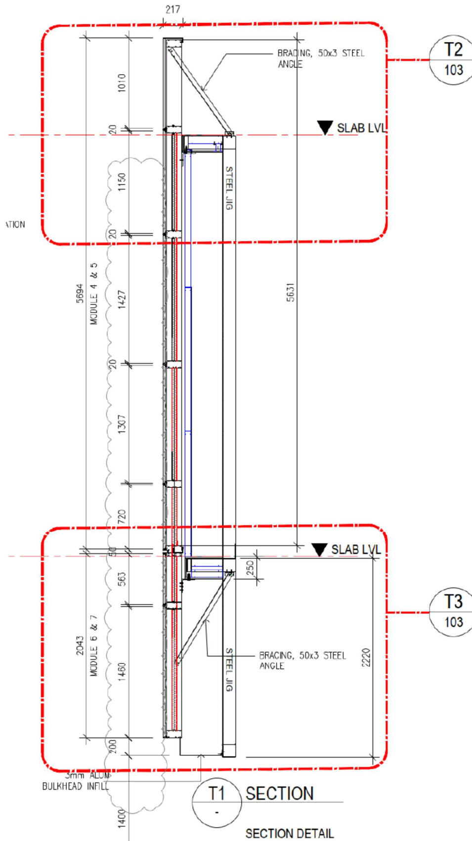
Figure 32 Vertical cross-section of the wing wall – with dimensions.
