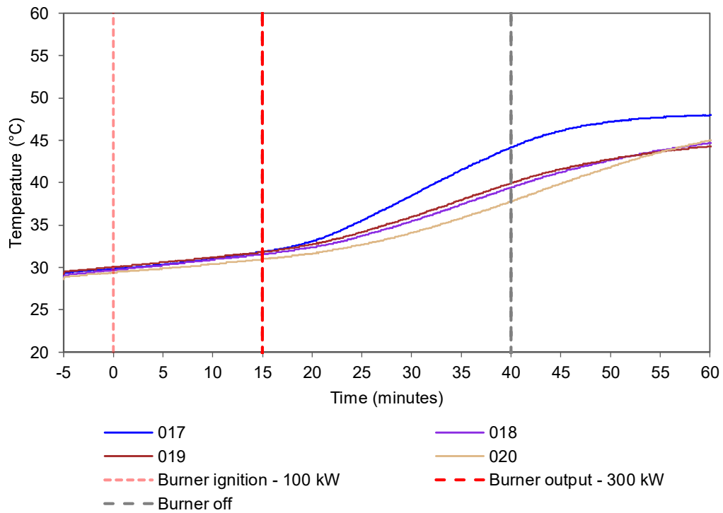
Figure 8 Internal temperatures of the back pan of module 3 - Temperature vs. time.
