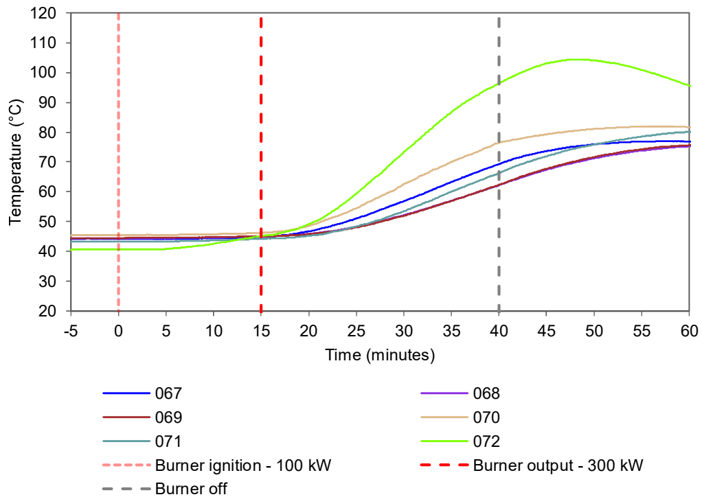
Figure 18 Internal temperatures of the back pan of module 7 - Temperature vs. time.
