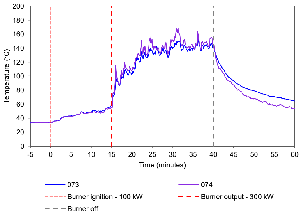
Figure 19 Internal temperatures of the cavity of module 6 - Temperature vs. time.
