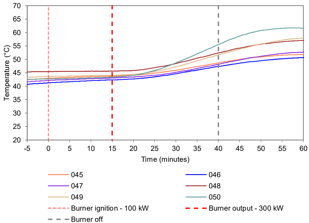
Figure 14 Internal temperatures of the back pan of module 5 (lower part) - Temperature vs. time.
