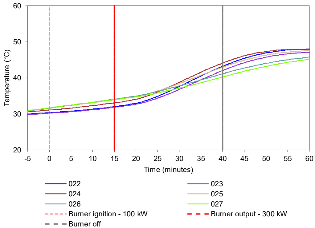
Figure 10 Internal temperatures of the back pan of module 4 (upper part) - Temperature vs. time.
