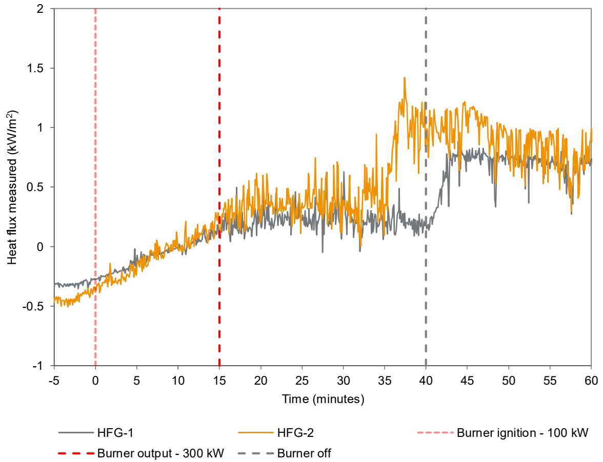
Figure 21 Measured heat flux data collected by the HFGs – Heat flux vs time.
