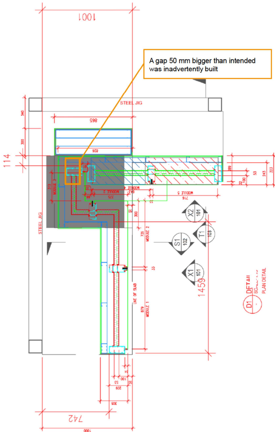
Figure 25 Plan view of the external wall – layout with dimensions.
