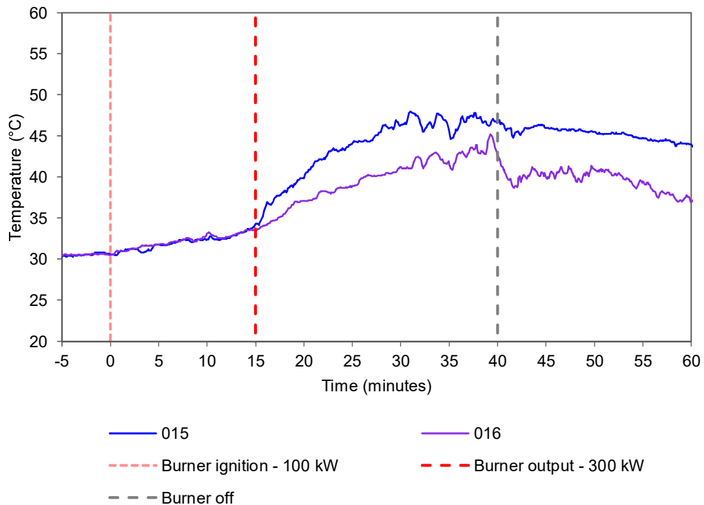
Figure 7 Internal temperatures of the cavity of module 2 - Temperature vs. time.
