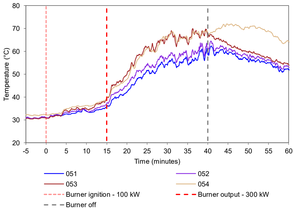
Figure 15 Internal temperatures of the cavity of module 5 - Temperature vs. time.
