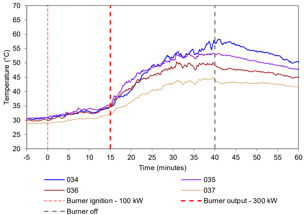
Figure 12 Internal temperatures of the cavity of module 4 - Temperature vs. time.
