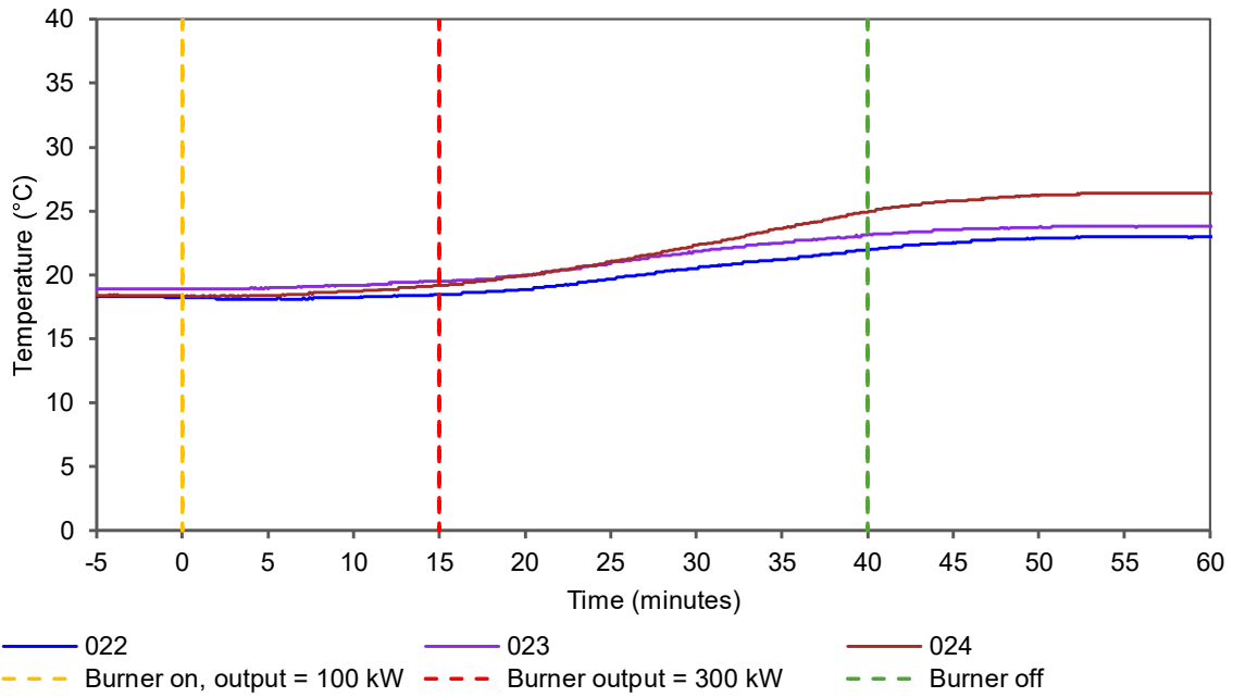
Figure 20 Internal temperatures located on the back pan on module 6 – temperature vs time
