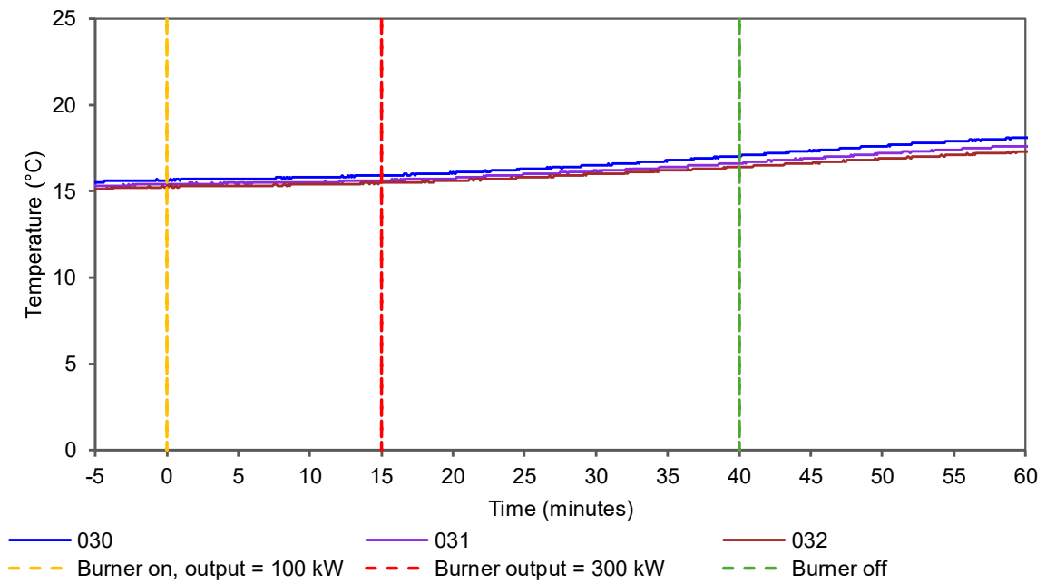
Figure 22 Internal temperatures located on the back pan on module 2 – temperature vs time
