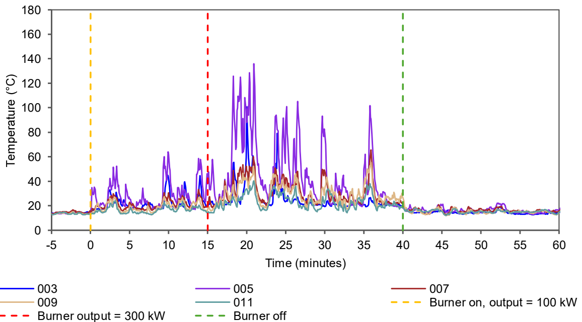
Figure 15 External surface temperatures at various heights on cladding away from the burner – temperature vs time
