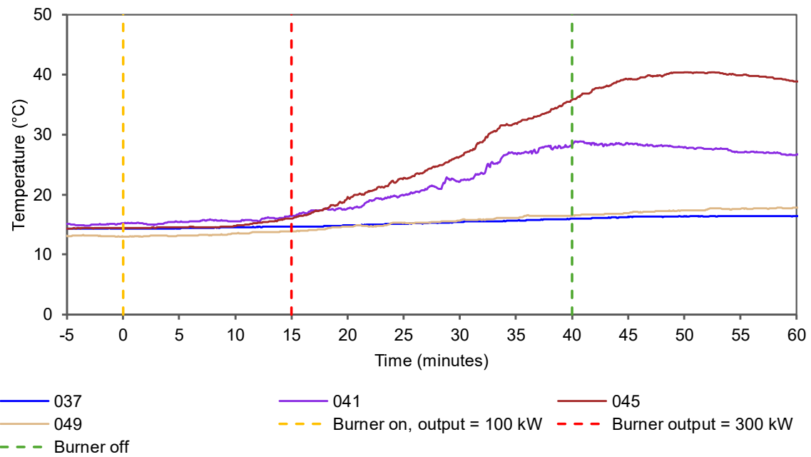
Figure 28 Cavity temperatures between the back pan and plasterboard of modules 1, 3, 5 and 7 – temperature vs time
