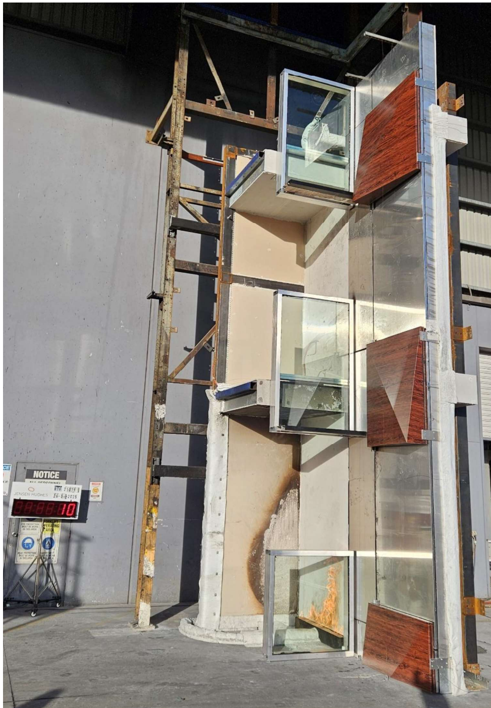
Figure 33 The specimen 10 minutes into the test with the burner at 100 kW.
