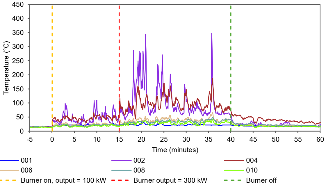
Figure 14 External surface temperatures at various heights on cladding close to the burner – temperature vs time
