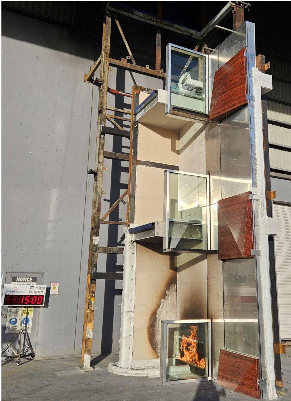
Figure 34 The specimen 15 minutes into the test – the burner output was increased to 300 kW.
