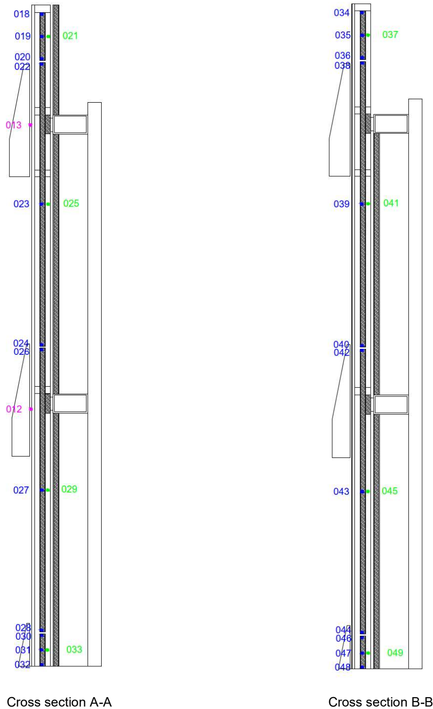
Figure 2 Instrumentation locations – Internal and cavity thermocouples - cross section A-A
