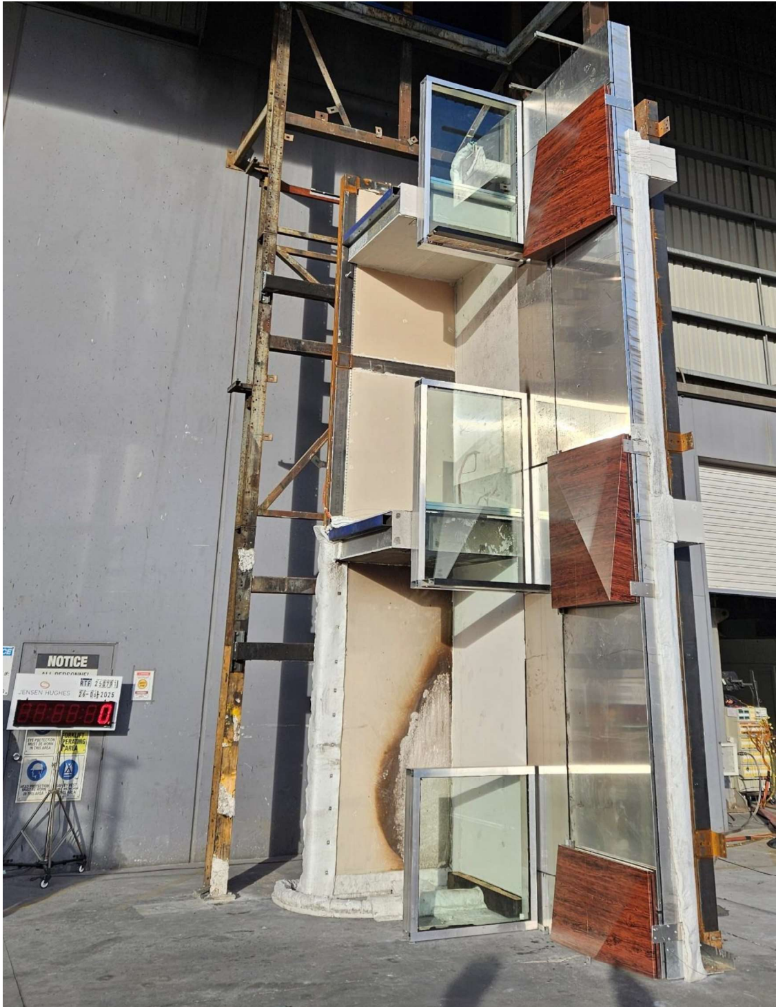
Figure 30 The specimen before the start of the test – exposed side
