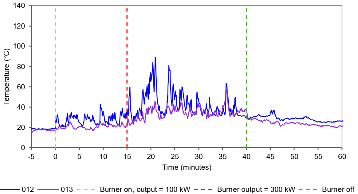
Figure 16 Cavity temperatures behind the 3D architectural modules – temperature vs time
