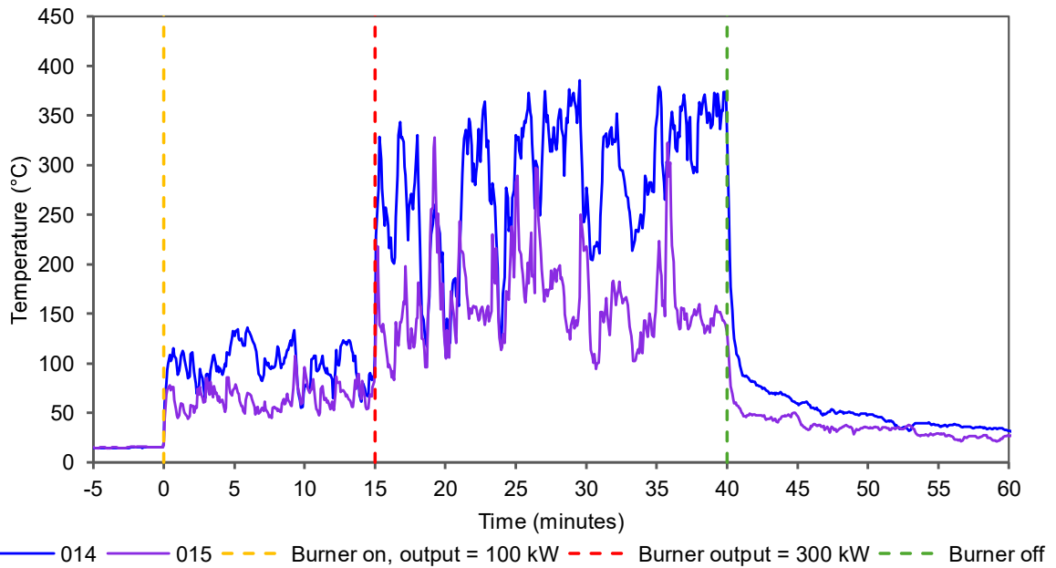
Figure 17 Surface temperature at level 1 balcony adjoining surfaces – temperature vs time
