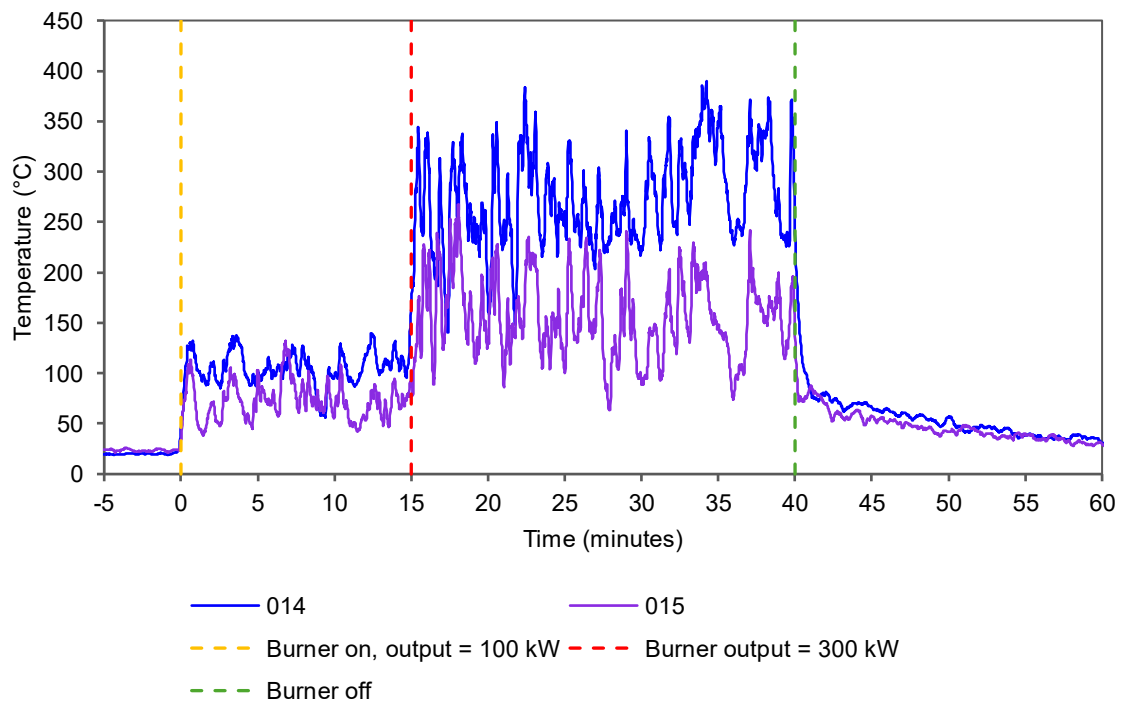
Figure 17 Surface temperature at level 1 balcony adjoining surfaces – temperature vs time
