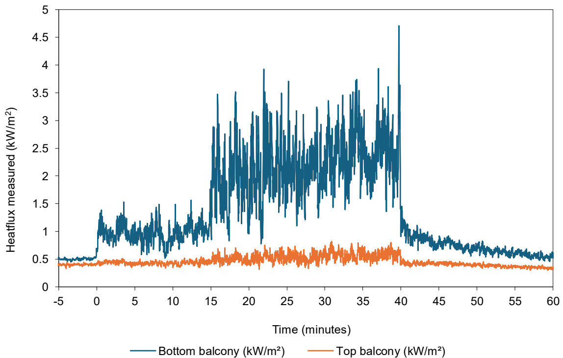
Figure 29 Measured heatflux data collected by the HFGs – Heat flux vs time
