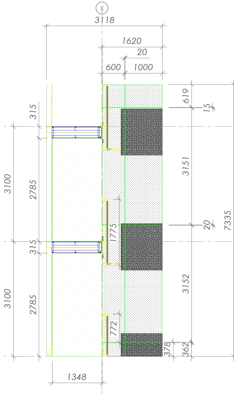
Figure 3 Elevation view of wing wall – ACP curtain wall overall measurements
