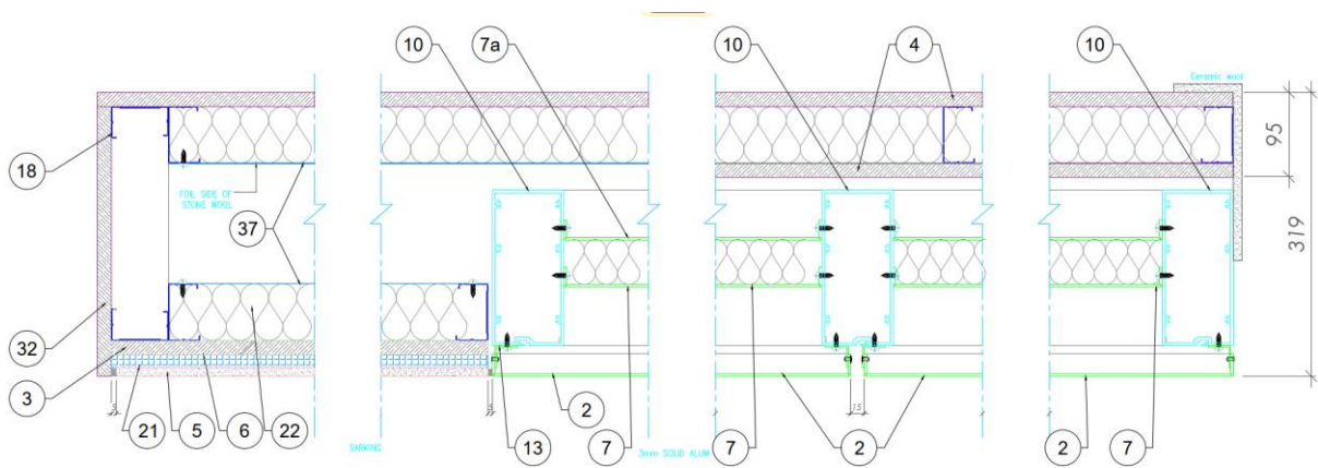
Figure 10 Balustrade section details
