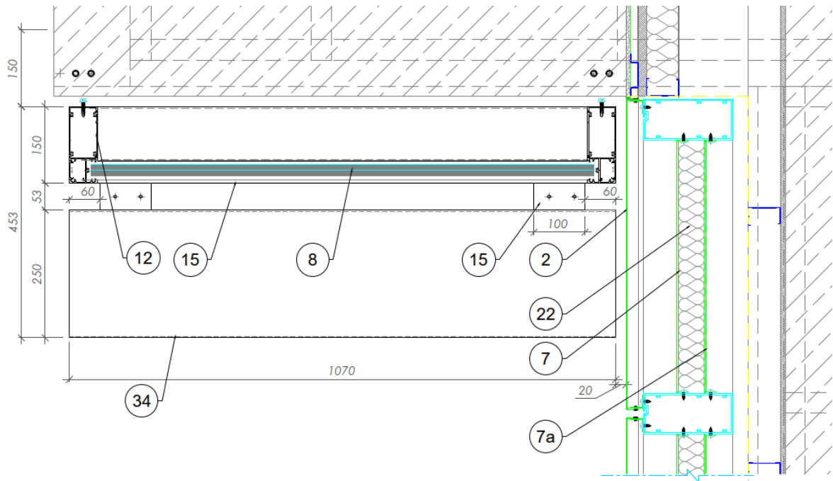
Figure 12 Balustrade plan details
