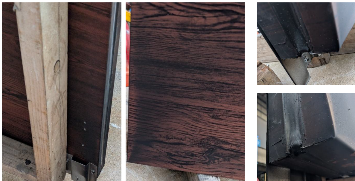
Figure 44 Post test condition of level 1 architectural module.
