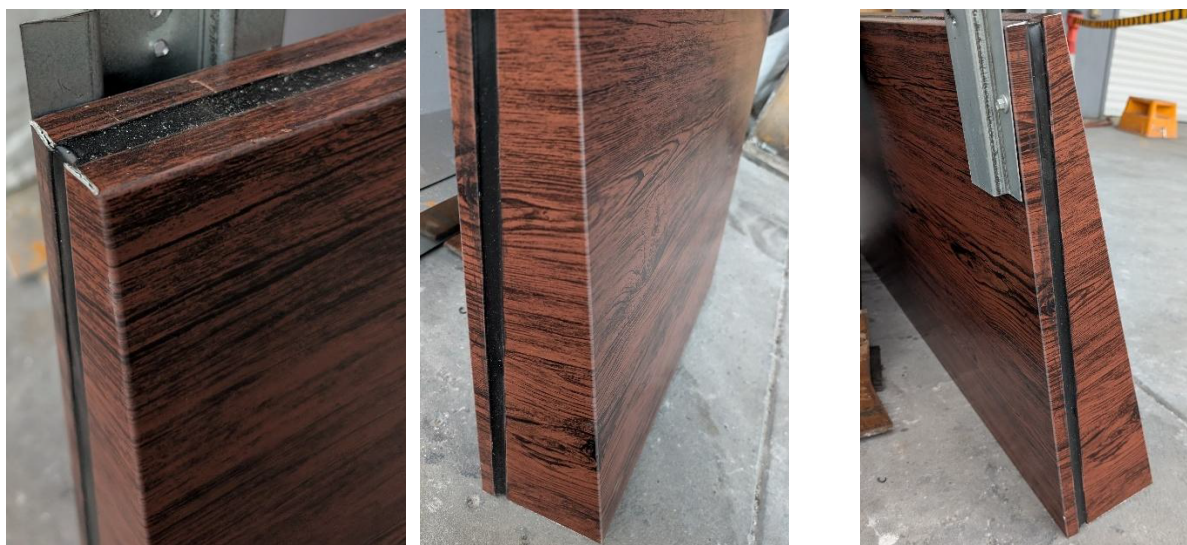
Figure 43 Post test condition of the ground level architectural module.
