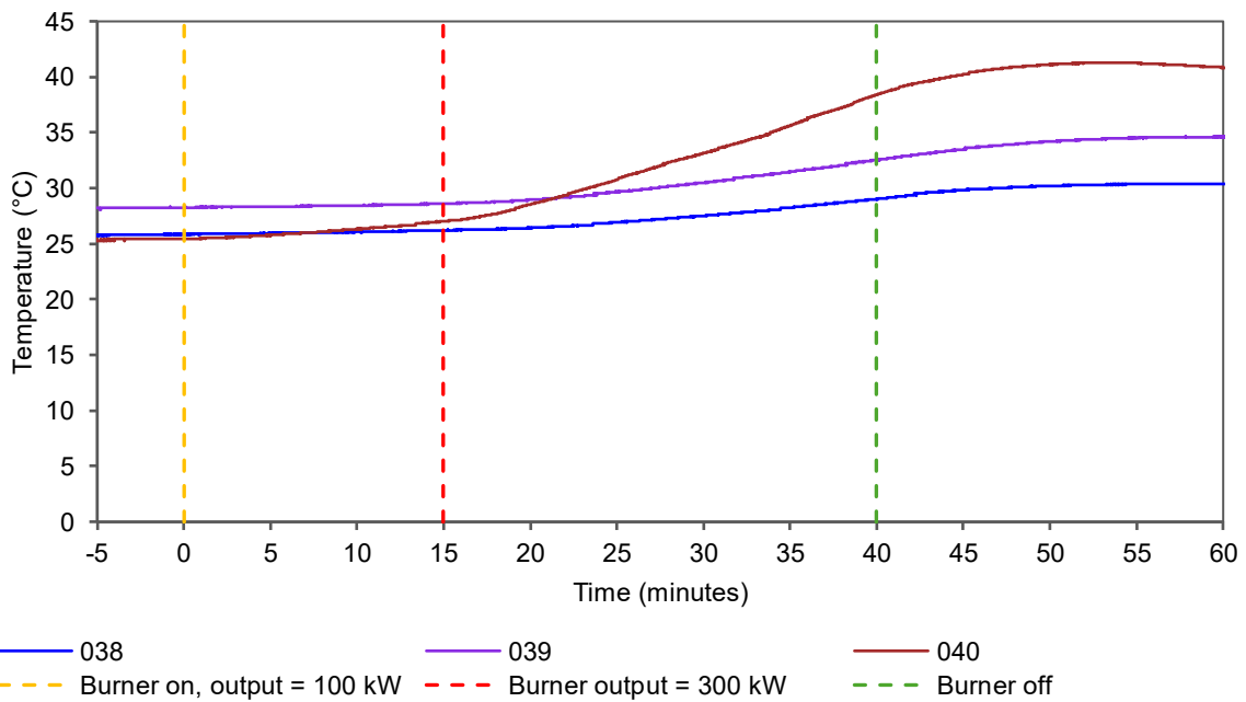
Figure 25 Internal temperatures located on the back pan on module 5 – temperature vs time
