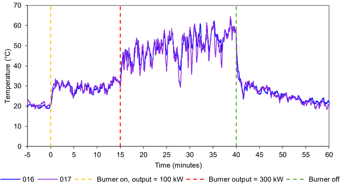
Figure 18 Surface temperature at level 2 balcony adjoining surfaces – temperature vs time
