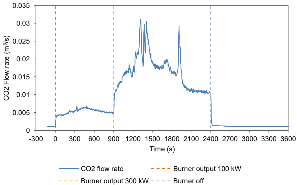
Figure 8 Production of carbon dioxide vs time, at reference temperature and pressure
