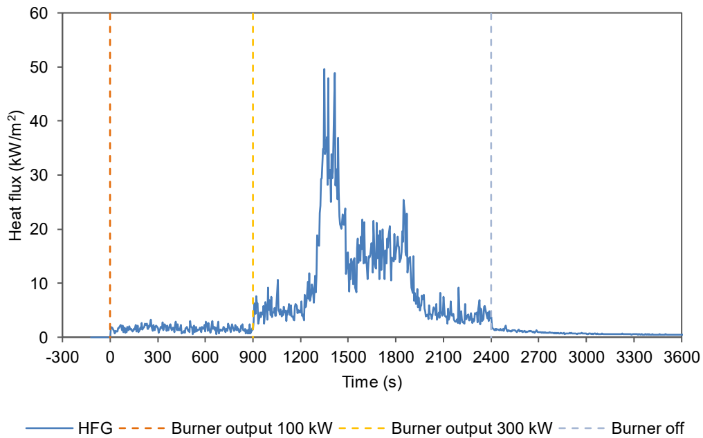
Figure 4 Heat flux vs time
