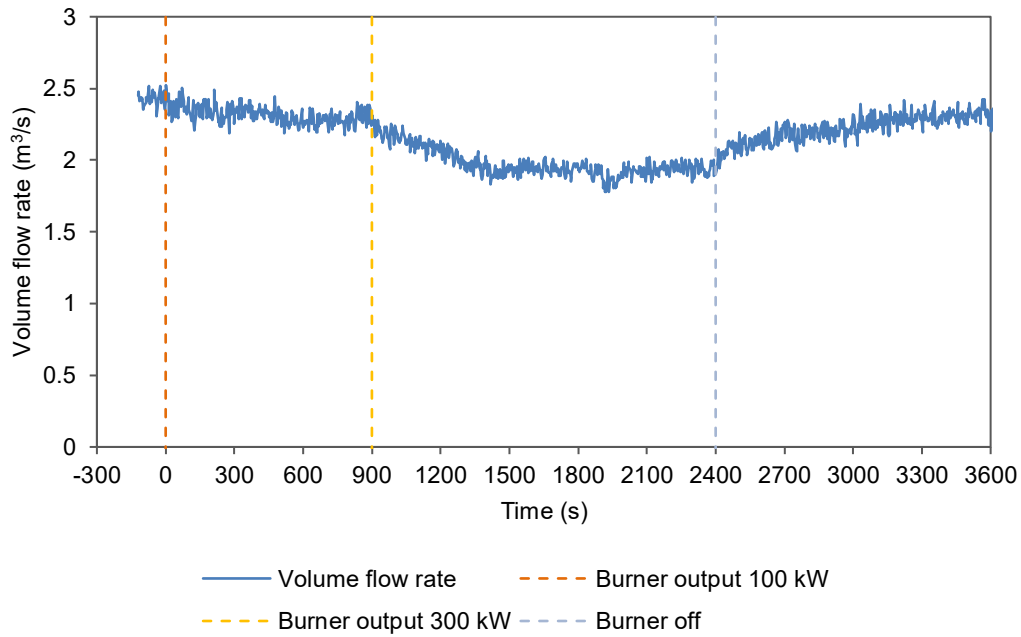
Figure 5 Volume flow rate in duct vs time
