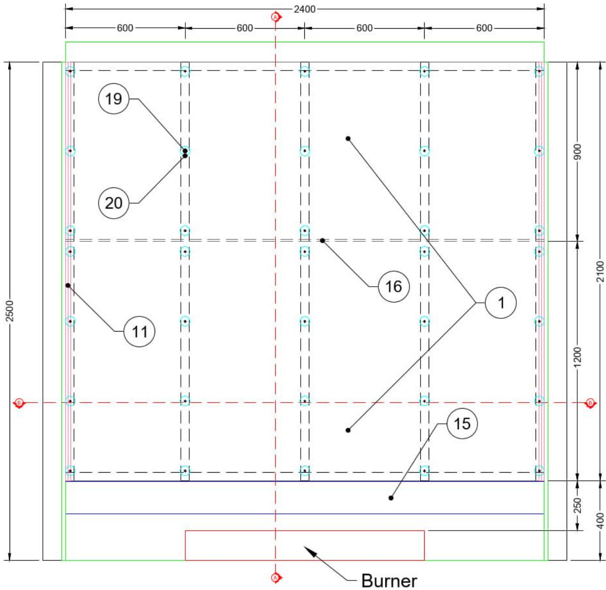
Figure 11 System assembly – Exposed side elevation
