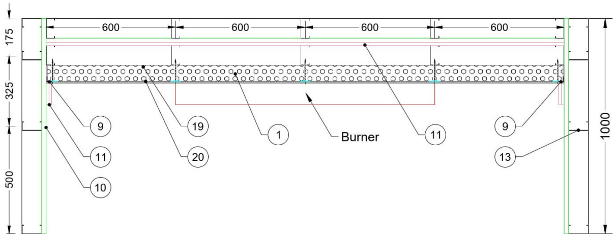
Figure 13 System assembly – Horizontal cross-section B-B
