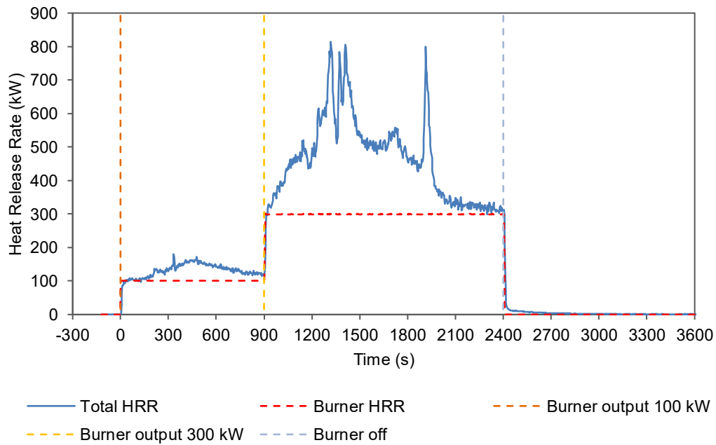
Figure 6 Heat release rate (HRR) of specimen and burner vs time
