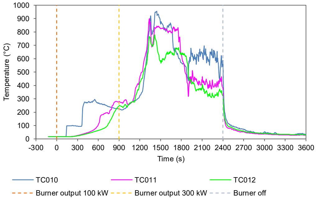
Figure 3 Embedded in the EPS, 40 mm from the unexposed face – Temperature vs time
