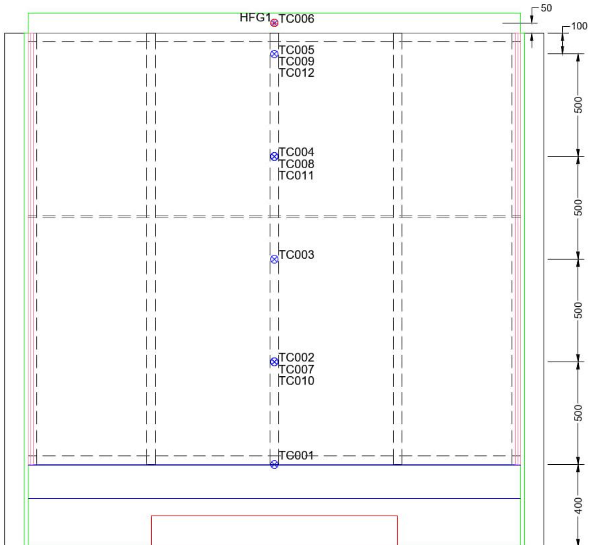
Figure 14 Instrumentation locations – Exposed side view
