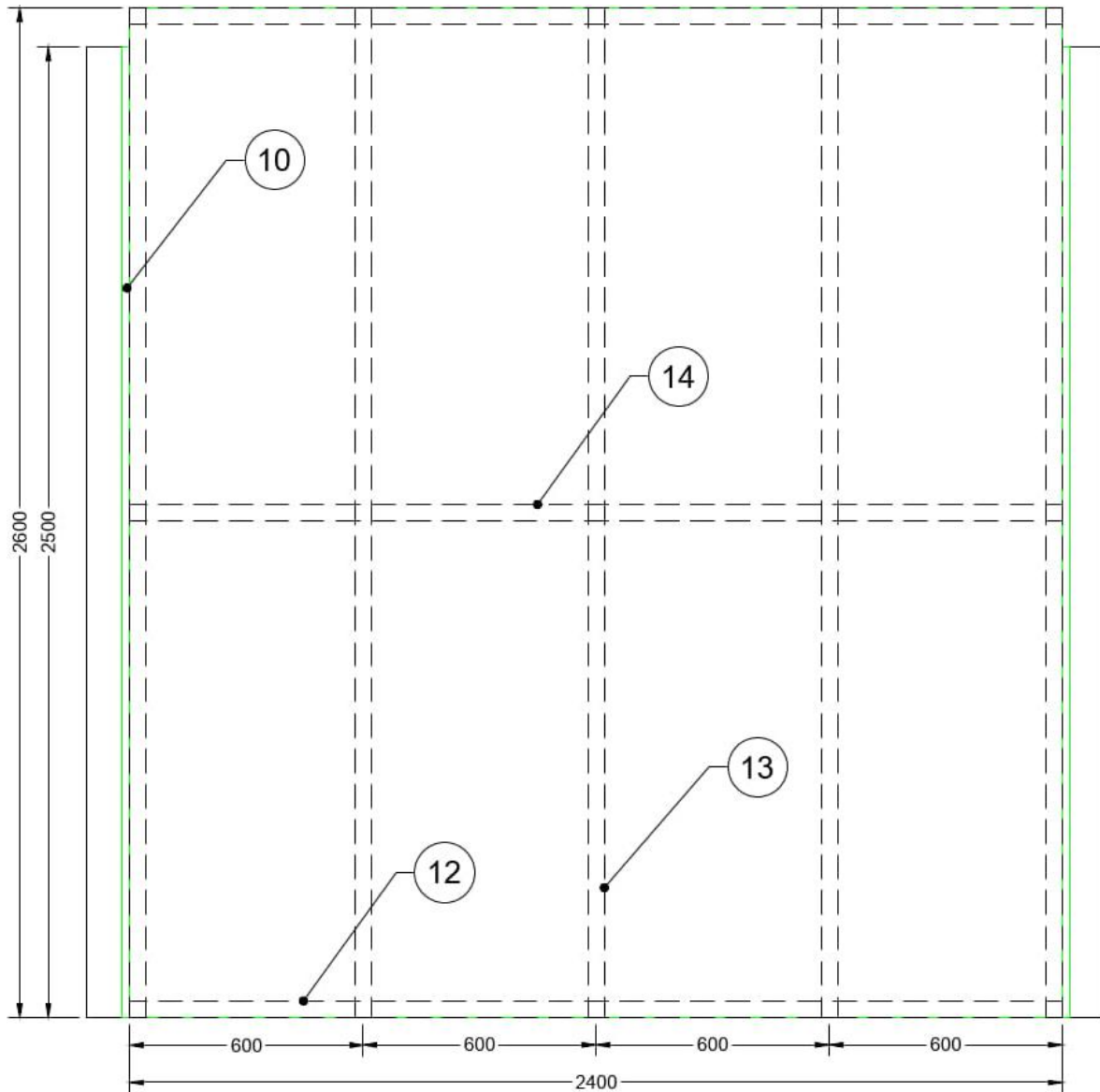
Figure 10 Elevation of rig support
