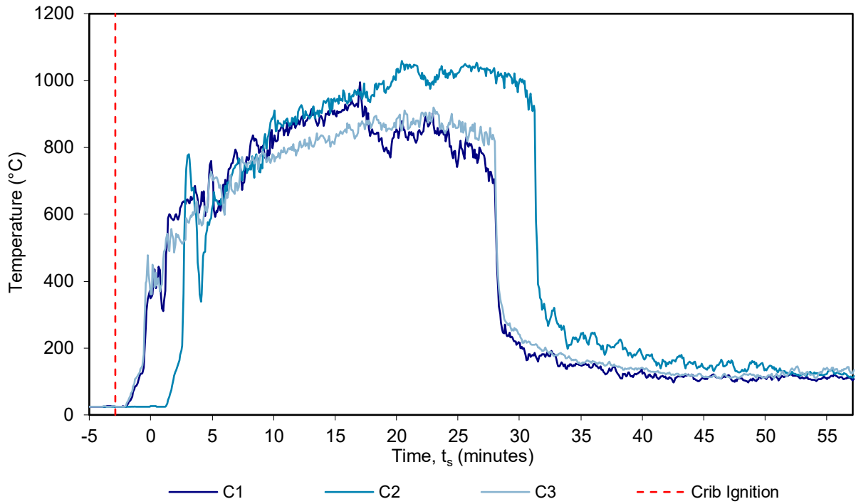
Figure 29 Combustion chamber – temperature vs time
