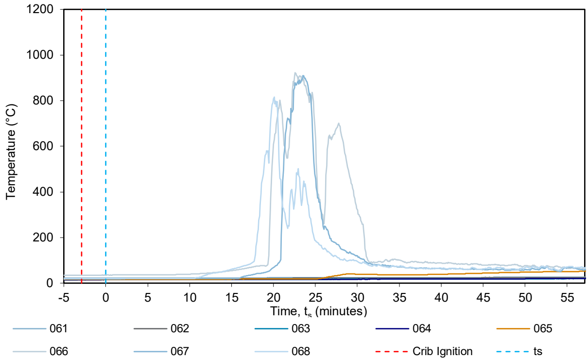
Figure 31 Stud MIMS, main wall – temperature vs time
