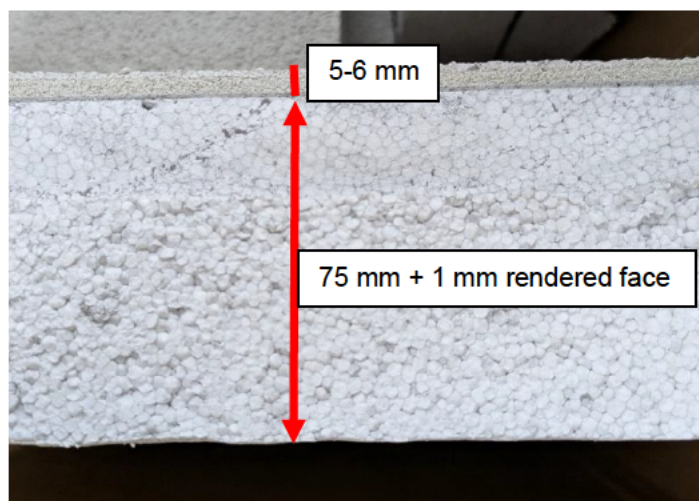
Figure 39 Cross section of the panel and thicknesses
