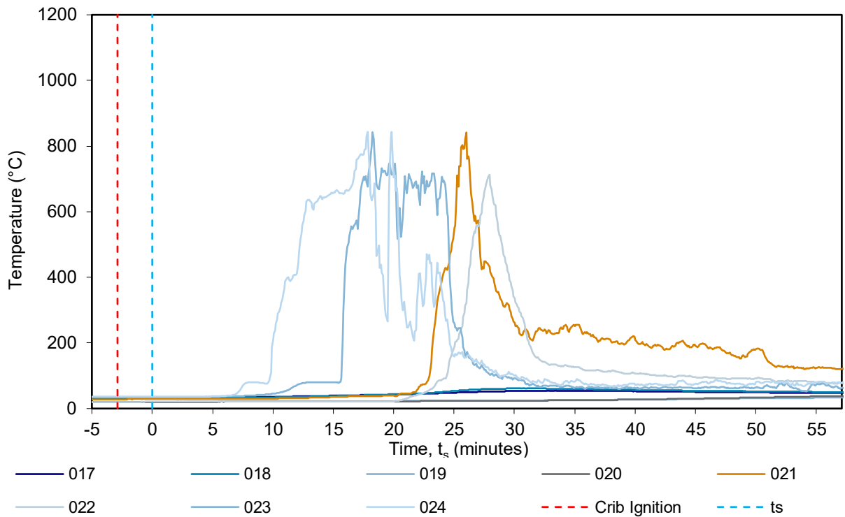
Figure 22 MIMS, main wall 2500 mm from the floor – temperature vs time
