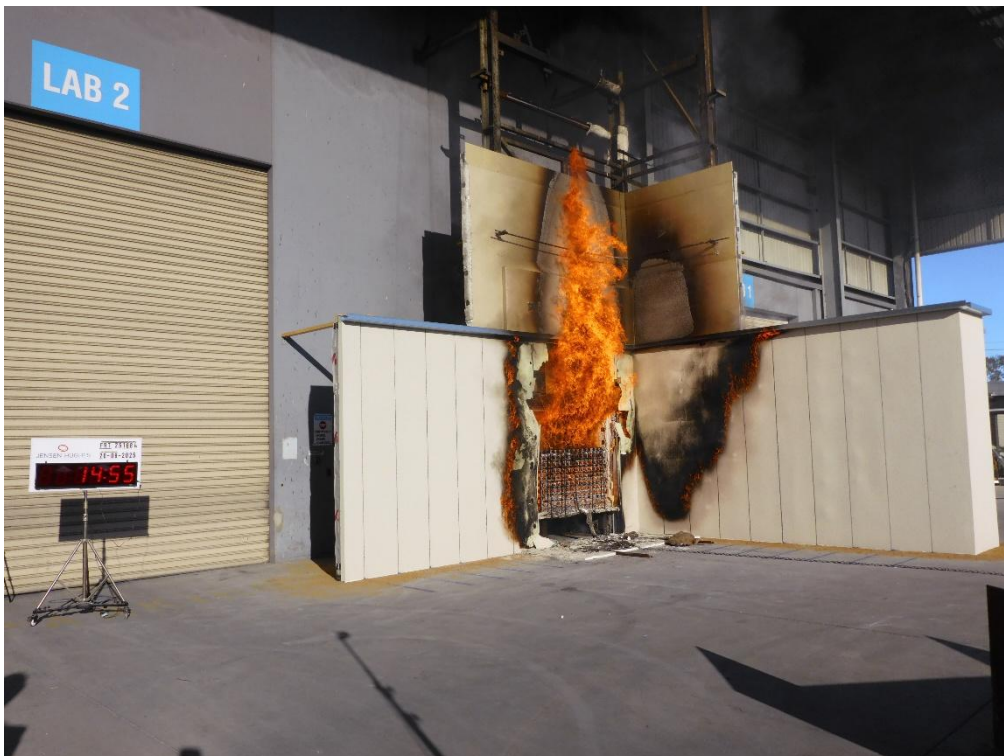
Figure 42 The wall system during the test – 14 minutes 55 seconds after crib ignition
