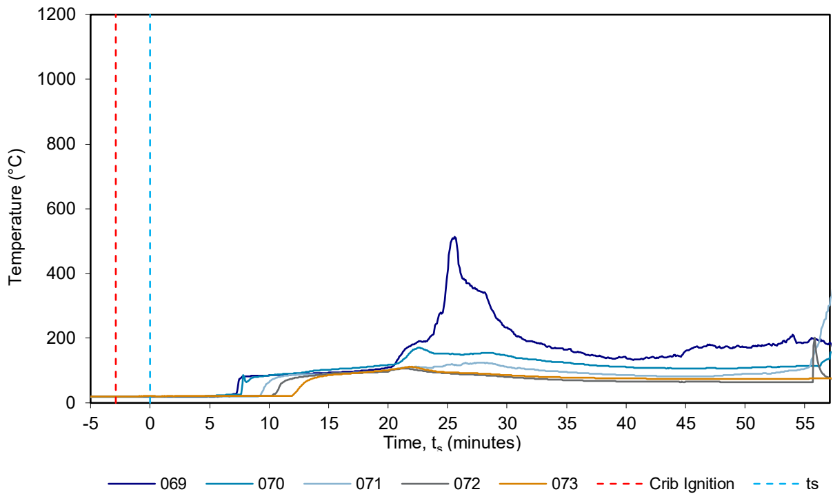
Figure 32 Stud MIMS, wing wall – temperature vs time
