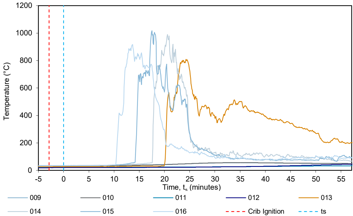
Figure 21 MIMS, main wall 1500 mm from the floor – temperature vs time
