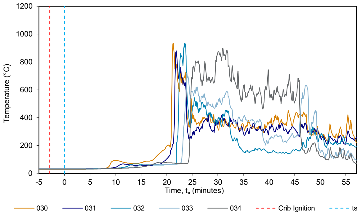
Figure 24 MIMS, wing wall 500 mm from the floor – temperature vs time
