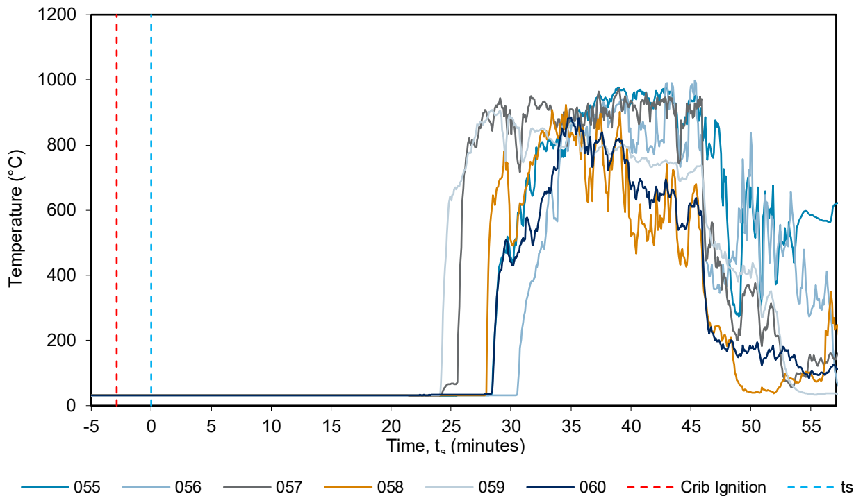
Figure 30 MIMS, return wall – temperature vs time
