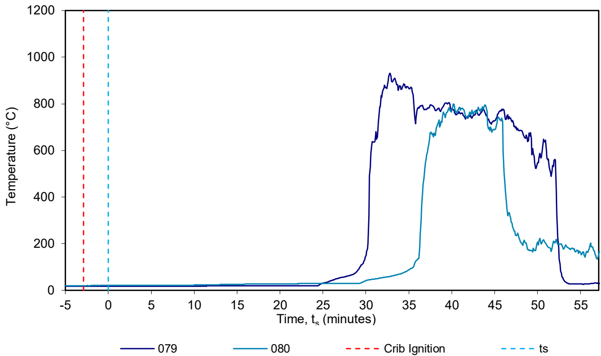
Figure 33 Stud MIMS, wing wall – temperature vs time
