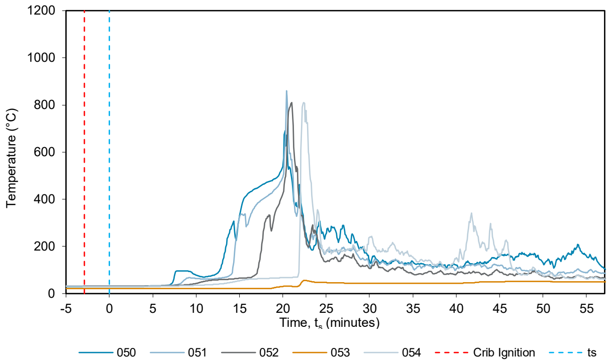
Figure 28 MIMS, wing wall 2500 mm from the floor – temperature vs time
