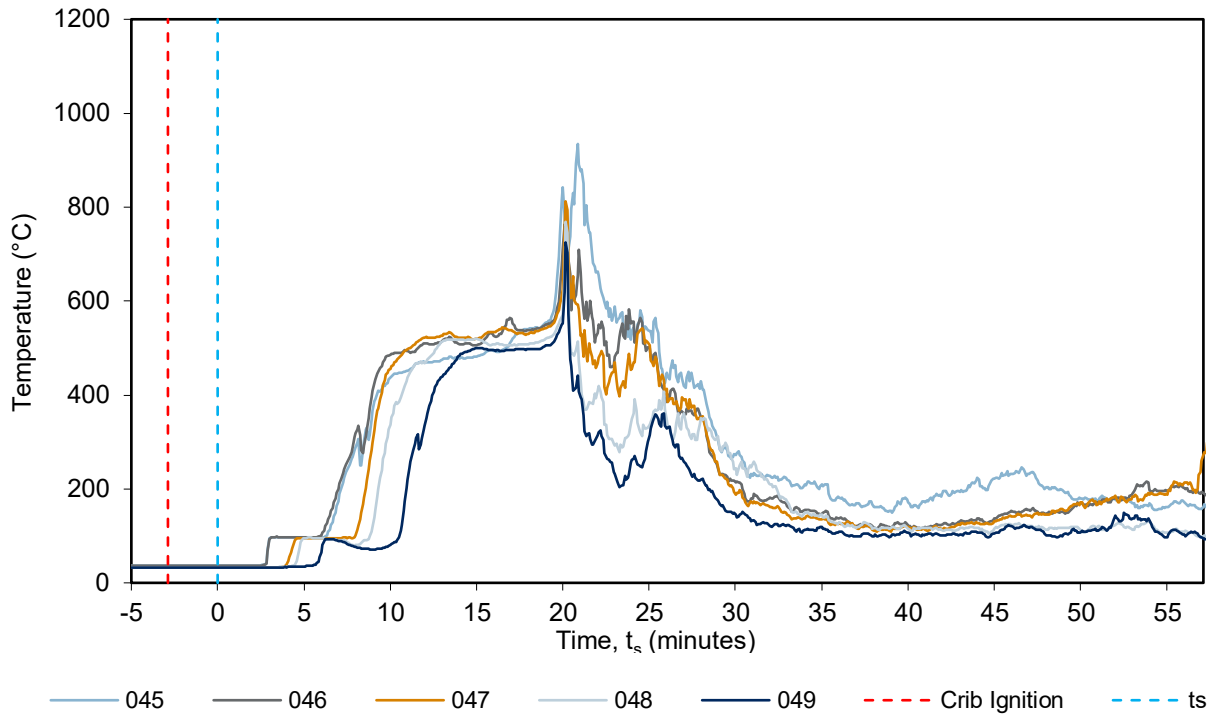
Figure 27 MIMS, wing wall 2500 mm from the floor – temperature vs time
