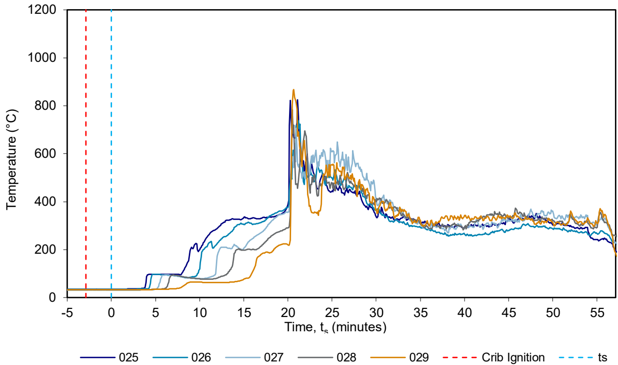
Figure 23 MIMS, wing wall 500 mm from the floor – temperature vs time
