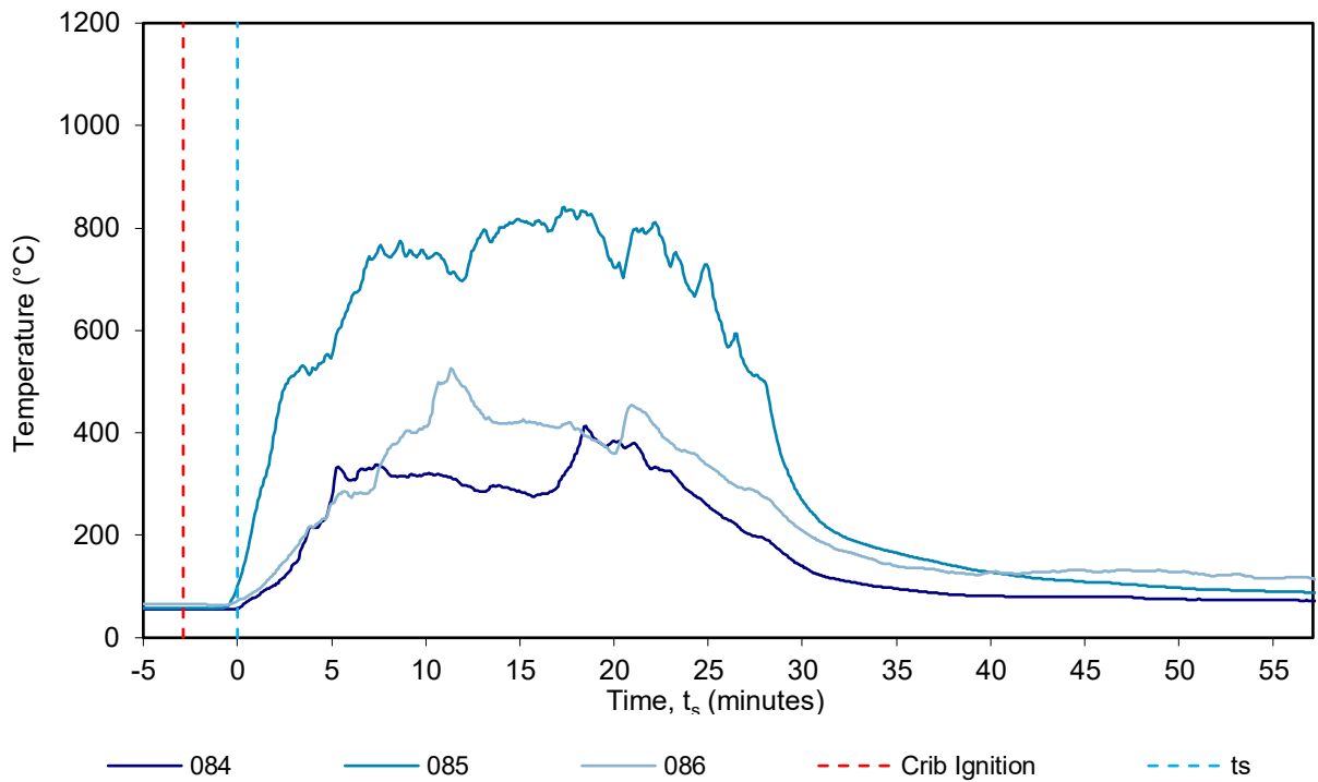
Figure 36 Plate thermometer – temperature vs time
