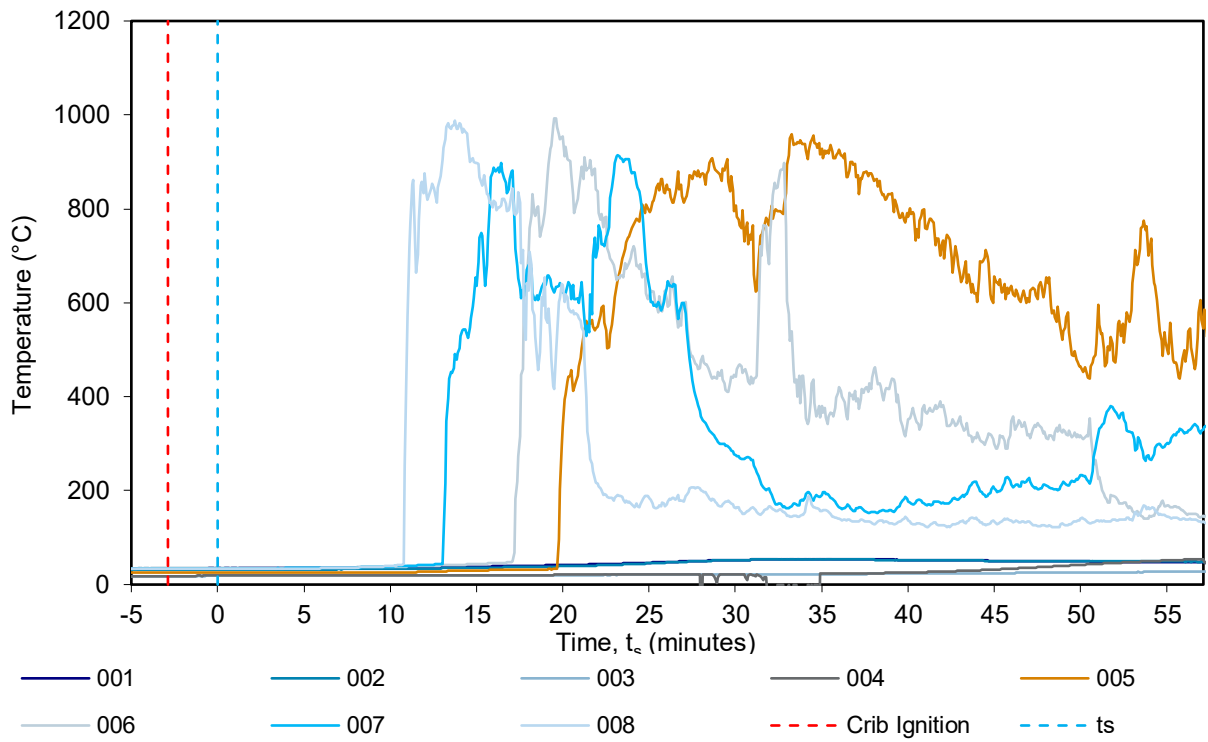
Figure 20 MIMS, main wall 500 mm from the floor – temperature vs time
