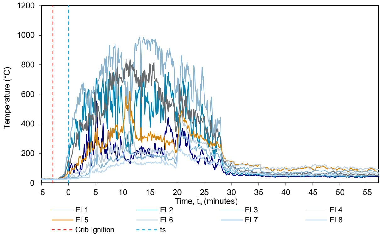
Figure 19 Level 1, external – temperature vs time
