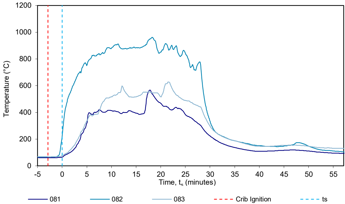
Figure 35 Plate thermometer – temperature vs time
