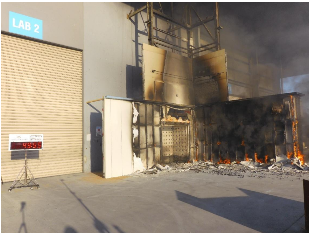
Figure 50 The wall system during the test – 49 minutes 55 seconds after crib ignition
