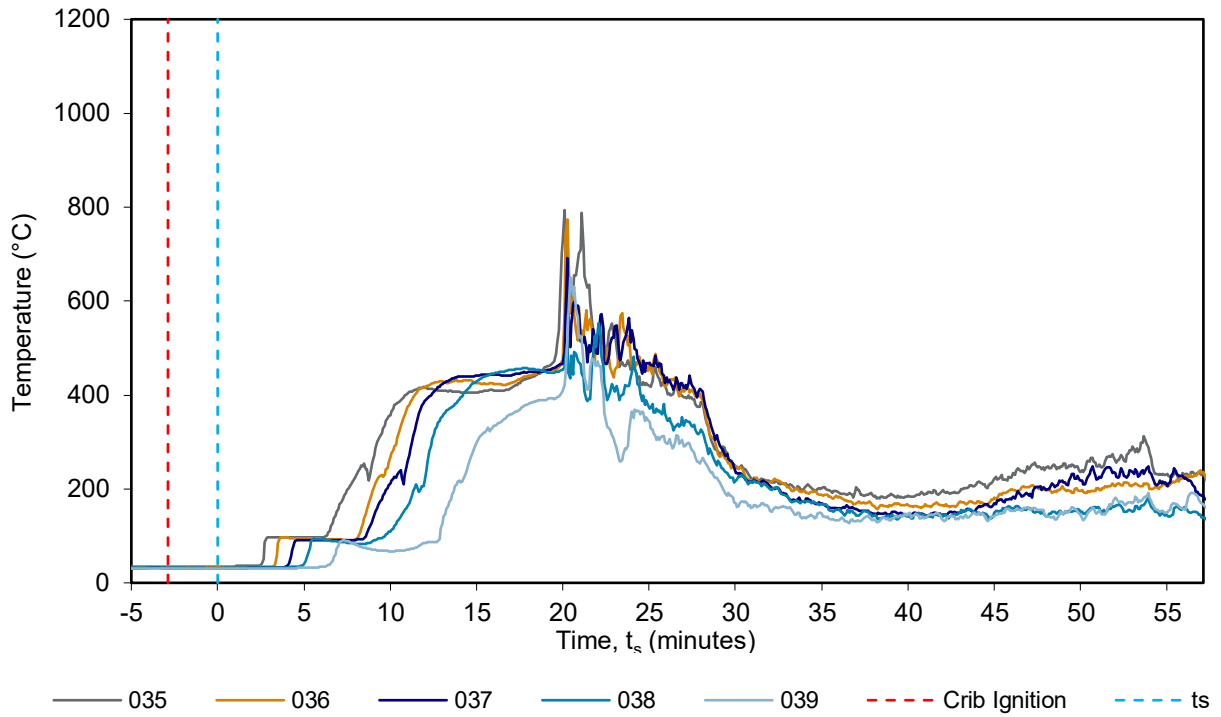
Figure 25 MIMS, wing wall 1500 mm from the floor – temperature vs time
