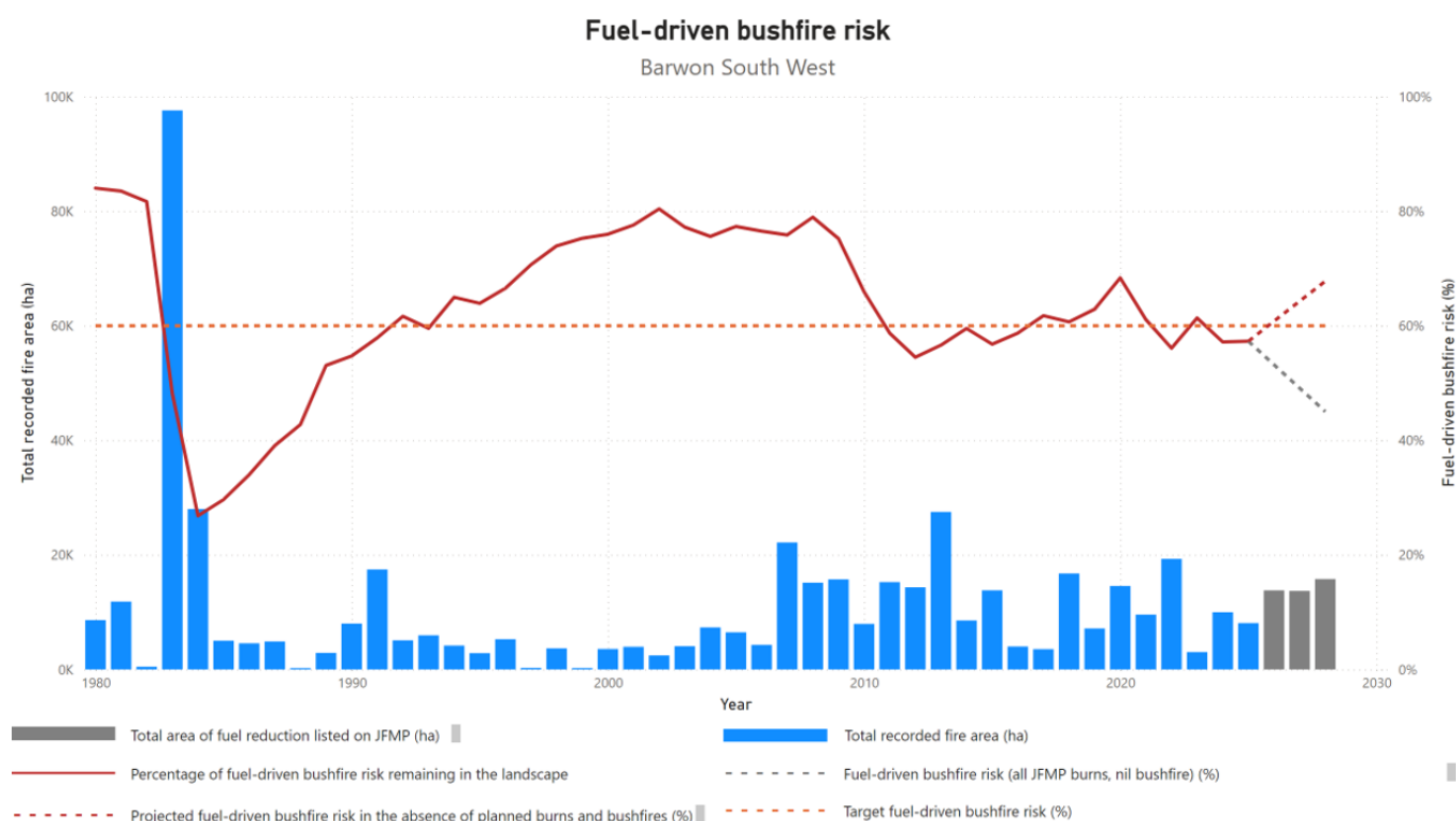
Figure 3: Barwon South West's fuel-driven bushfire risk from 1980-2025.
