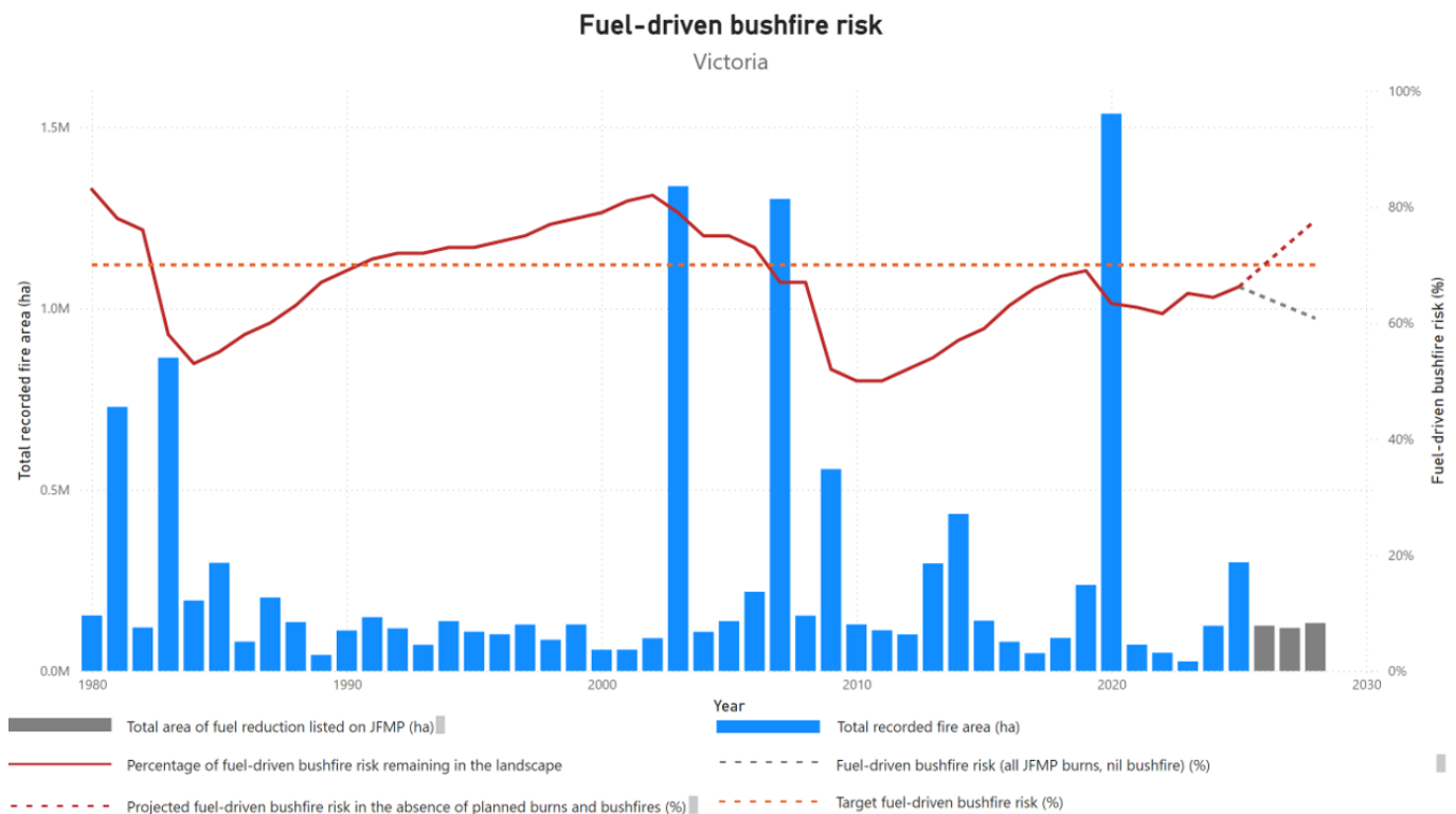
Figure 2: Victoria's fuel-driven bushfire risk from 1980-2025
